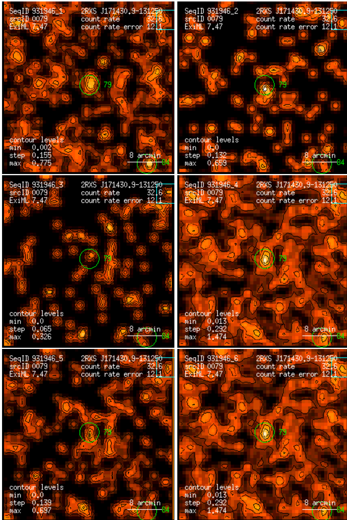
Figure 79: RASS 931946: detection 0079: band rate images, Gaussian filter: (1) PSPC channels 11 – 41, (2) 52 – 90, (3) 91 – 201, (4) 11 – 235, (5) 52 – 201, (6) 11 – 201. Broad band rates in counts/ks. Band rate contour levels in counts/ks/arcmin 2 .
