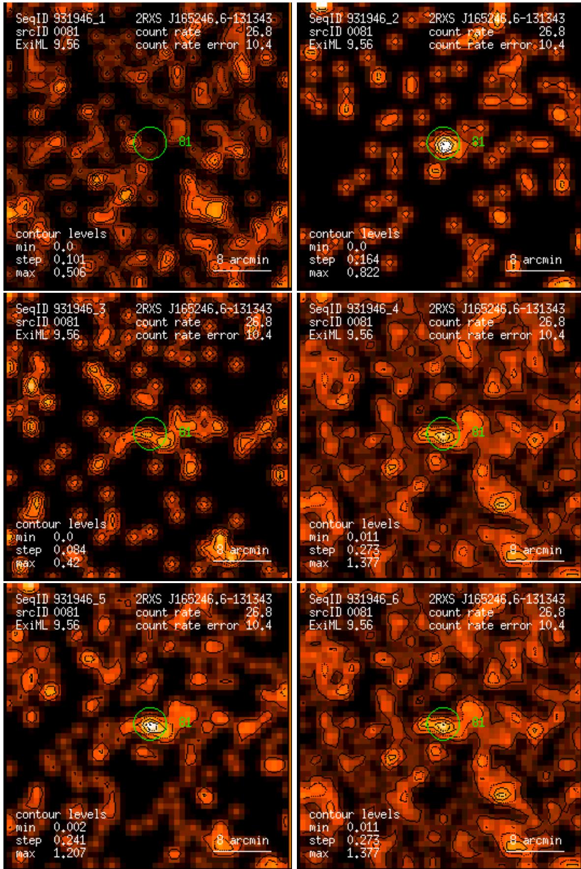
Figure 81: RASS 931946: detection 0081: band rate images, Gaussian filter: (1) PSPC channels 11 – 41, (2) 52 – 90, (3) 91 – 201, (4) 11 – 235, (5) 52 – 201, (6) 11 – 201. Broad band rates in counts/ks. Band rate contour levels in counts/ks/arcmin 2 .
