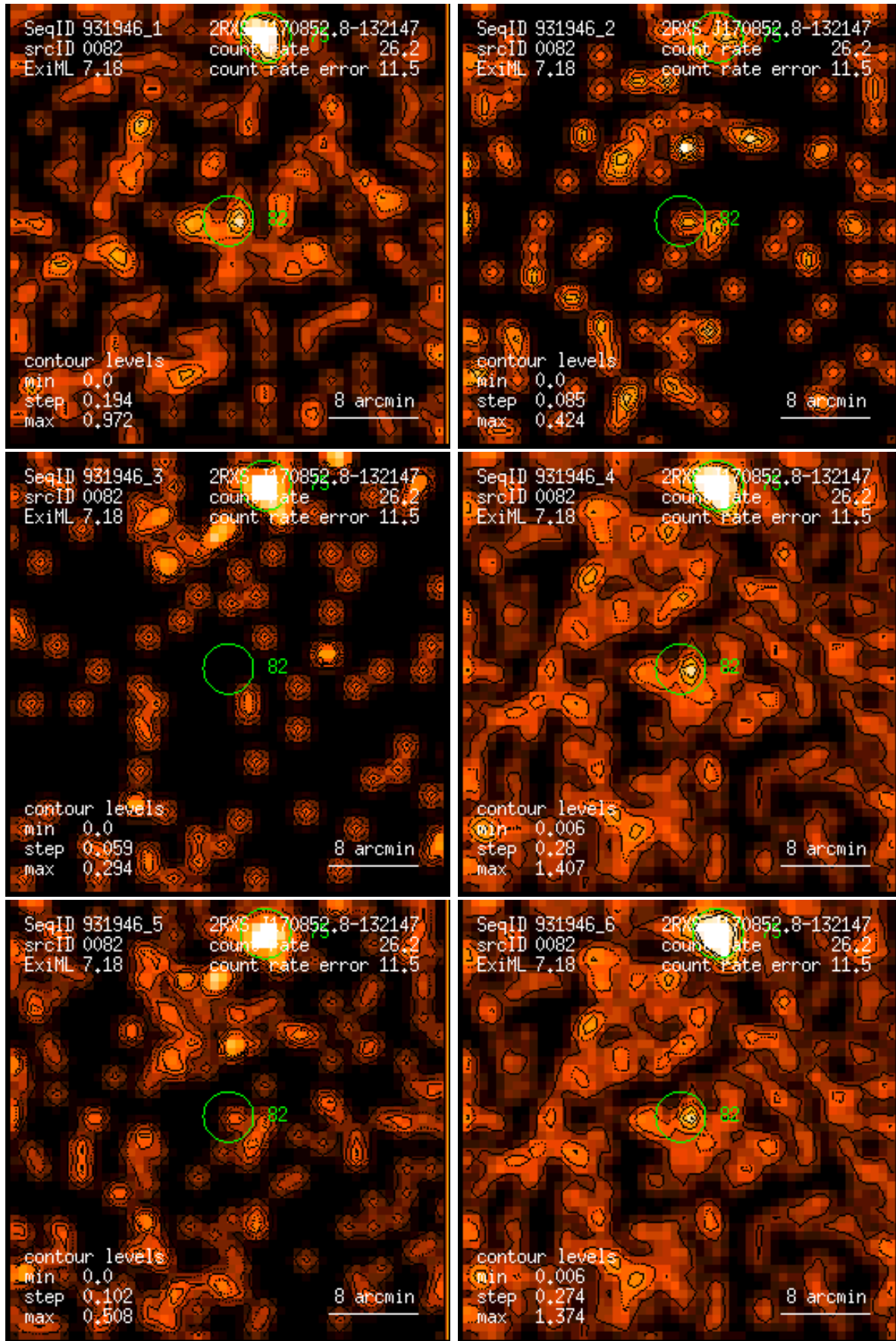
Figure 82: RASS 931946: detection 0082: band rate images, Gaussian filter: (1) PSPC channels 11 – 41, (2) 52 – 90, (3) 91 – 201, (4) 11 – 235, (5) 52 – 201, (6) 11 – 201. Broad band rates in counts/ks. Band rate contour levels in counts/ks/arcmin 2 .
