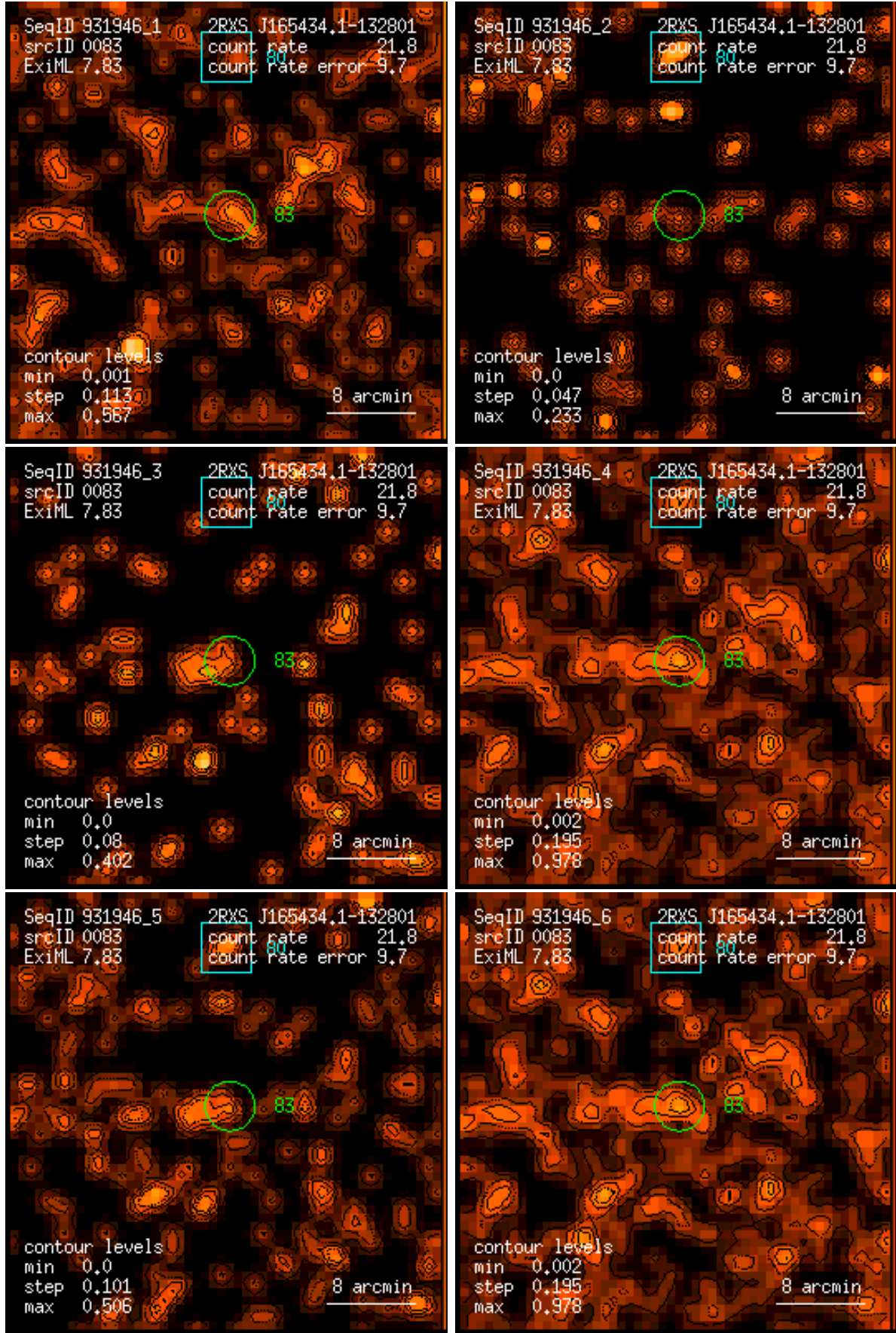
Figure 83: RASS 931946: detection 0083: band rate images, Gaussian filter: (1) PSPC channels 11 – 41, (2) 52 – 90, (3) 91 – 201, (4) 11 – 235, (5) 52 – 201, (6) 11 – 201. Broad band rates in counts/ks. Band rate contour levels in counts/ks/arcmin 2 .
