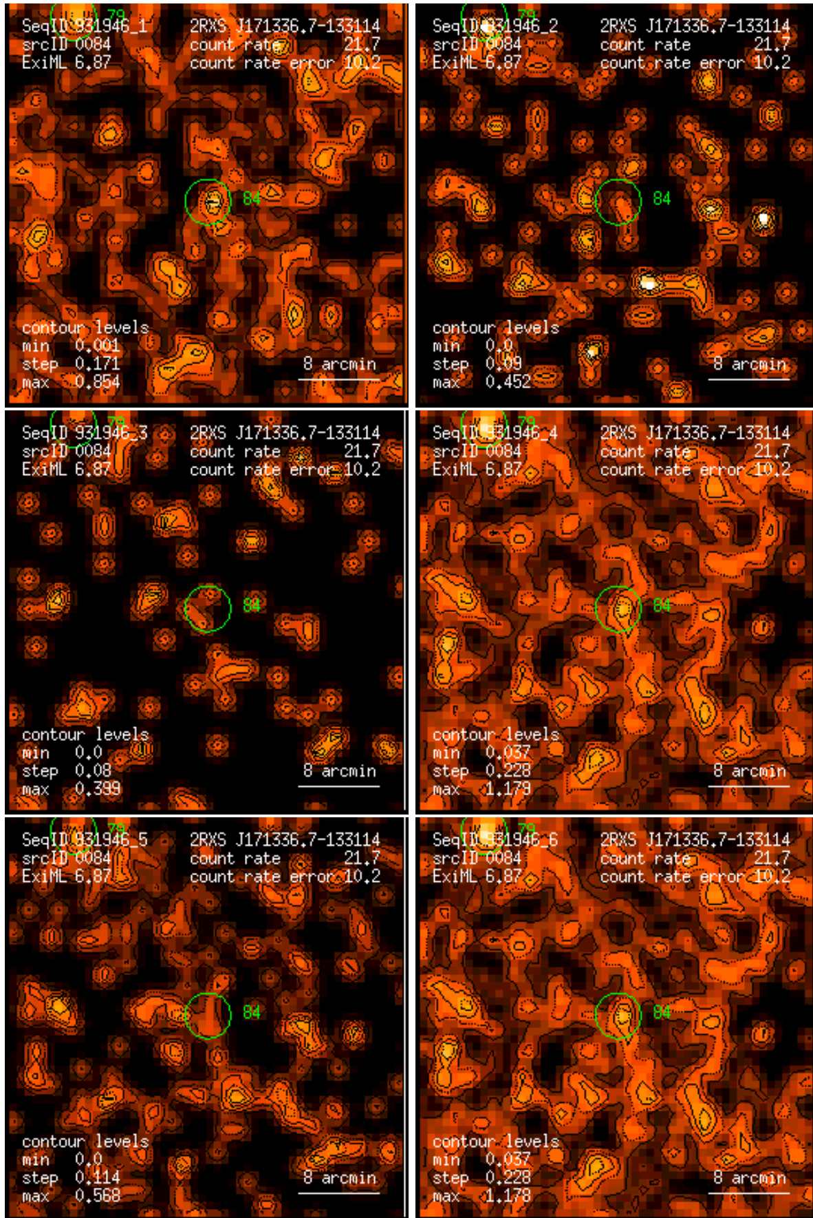
Figure 84: RASS 931946: detection 0084: band rate images, Gaussian filter: (1) PSPC channels 11 – 41, (2) 52 – 90, (3) 91 – 201, (4) 11 – 235, (5) 52 – 201, (6) 11 – 201. Broad band rates in counts/ks. Band rate contour levels in counts/ks/arcmin 2 .
