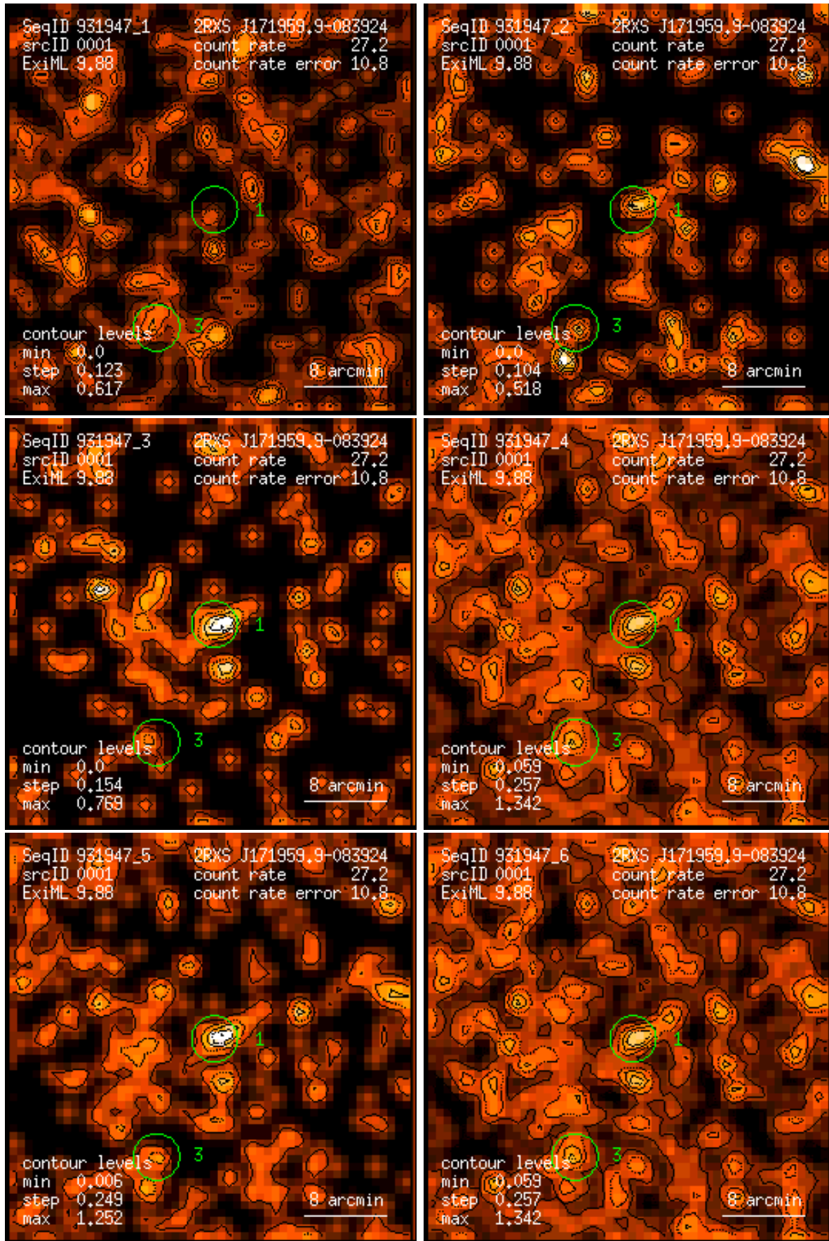
Figure 1: RASS 931947: detection 0001: band rate images, Gaussian filter: (1) PSPC channels 11 – 41, (2) 52 – 90, (3) 91 – 201, (4) 11 – 235, (5) 52 – 201, (6) 11 – 201. Broad band rates in counts/ks. Band rate contour levels in counts/ks/arcmin 2 .
