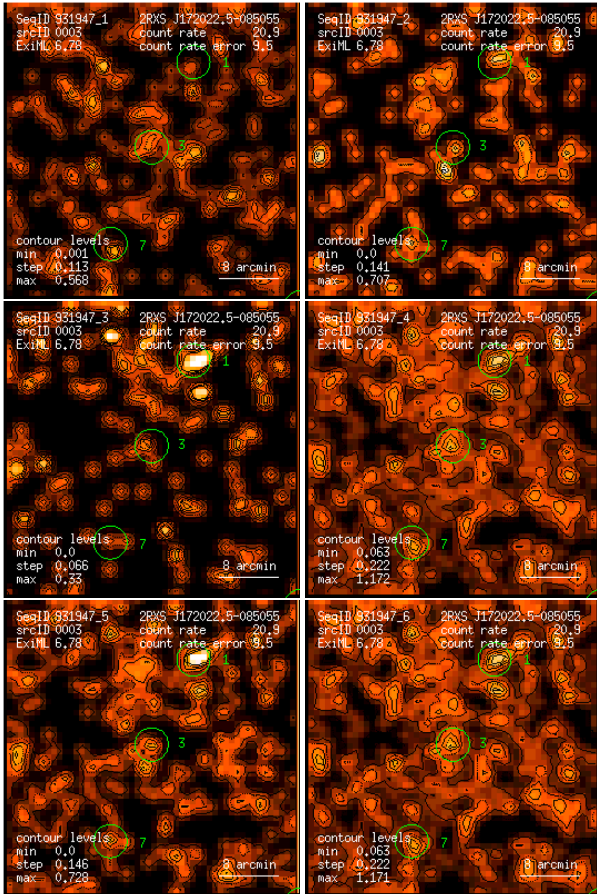
Figure 3: RASS 931947: detection 0003: band rate images, Gaussian filter: (1) PSPC channels 11 – 41, (2) 52 – 90, (3) 91 – 201, (4) 11 – 235, (5) 52 – 201, (6) 11 – 201. Broad band rates in counts/ks. Band rate contour levels in counts/ks/arcmin 2 .
