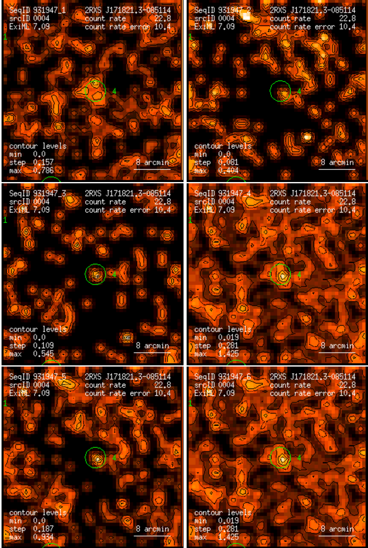
Figure 4: RASS 931947: detection 0004: band rate images, Gaussian filter: (1) PSPC channels 11 – 41, (2) 52 – 90, (3) 91 – 201, (4) 11 – 235, (5) 52 – 201, (6) 11 – 201. Broad band rates in counts/ks. Band rate contour levels in counts/ks/arcmin 2 .
