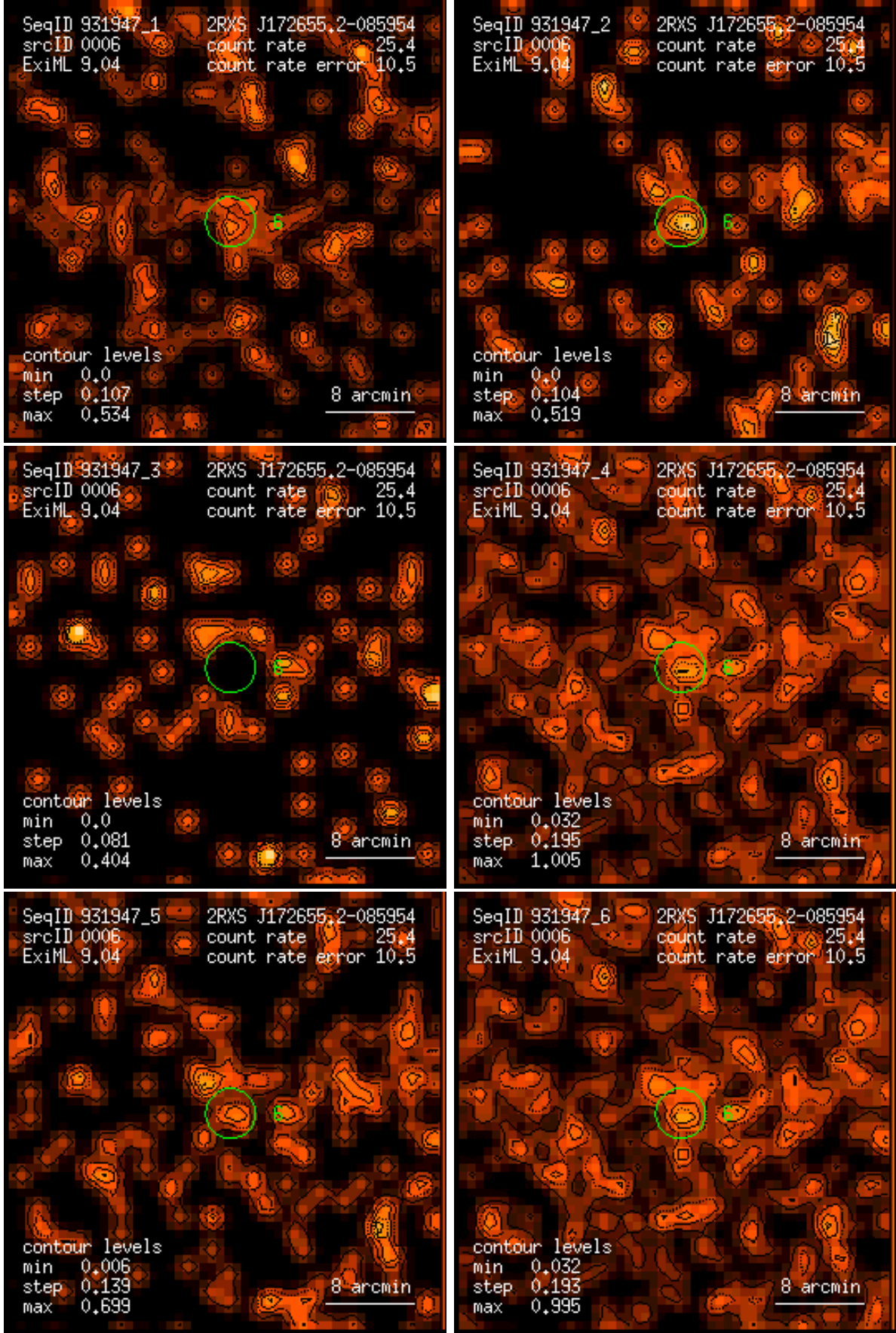
Figure 6: RASS 931947: detection 0006: band rate images, Gaussian filter: (1) PSPC channels 11 – 41, (2) 52 – 90, (3) 91 – 201, (4) 11 – 235, (5) 52 – 201, (6) 11 – 201. Broad band rates in counts/ks. Band rate contour levels in counts/ks/arcmin 2 .
