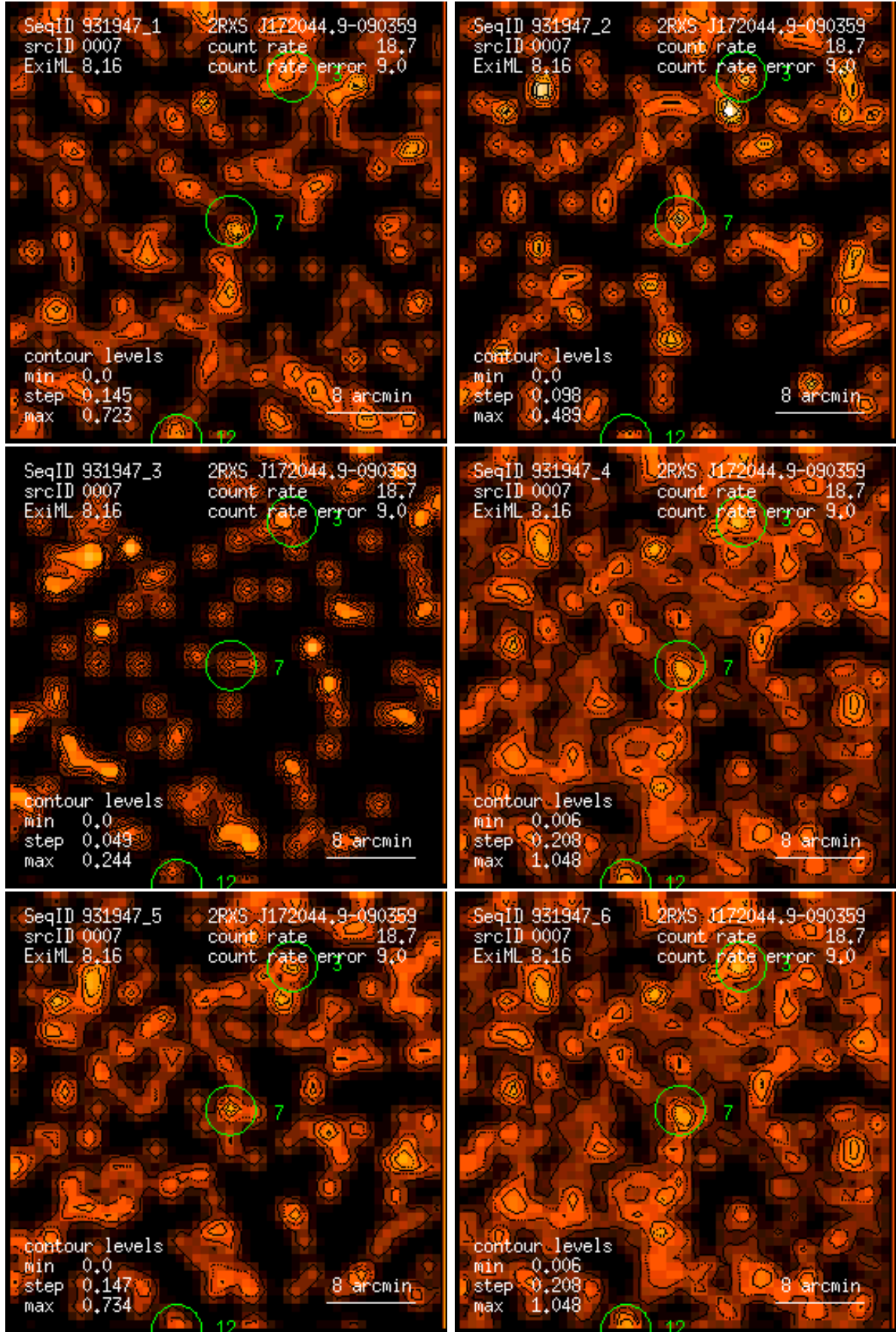
Figure 7: RASS 931947: detection 0007: band rate images, Gaussian filter: (1) PSPC channels 11 – 41, (2) 52 – 90, (3) 91 – 201, (4) 11 – 235, (5) 52 – 201, (6) 11 – 201. Broad band rates in counts/ks. Band rate contour levels in counts/ks/arcmin 2 .
