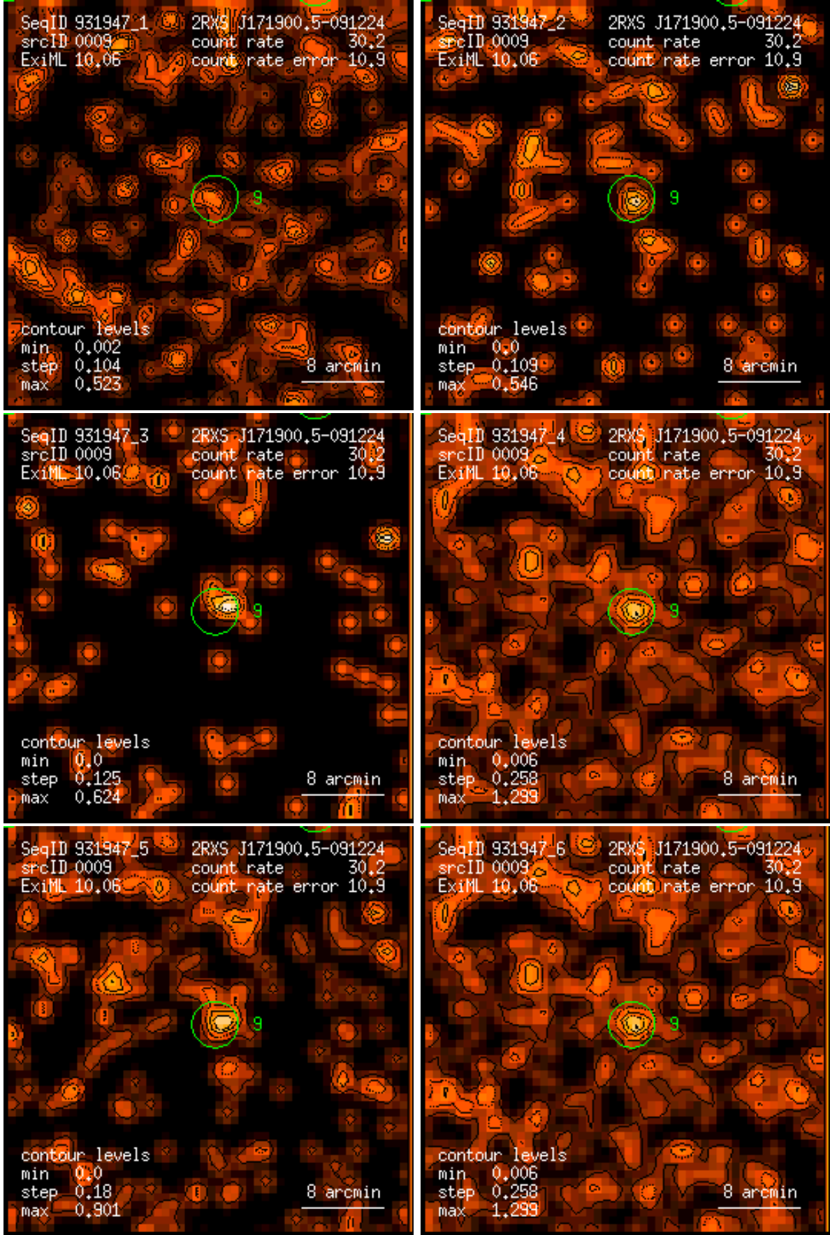
Figure 9: RASS 931947: detection 0009: band rate images, Gaussian filter: (1) PSPC channels 11 – 41, (2) 52 – 90, (3) 91 – 201, (4) 11 – 235, (5) 52 – 201, (6) 11 – 201. Broad band rates in counts/ks. Band rate contour levels in counts/ks/arcmin 2 .
