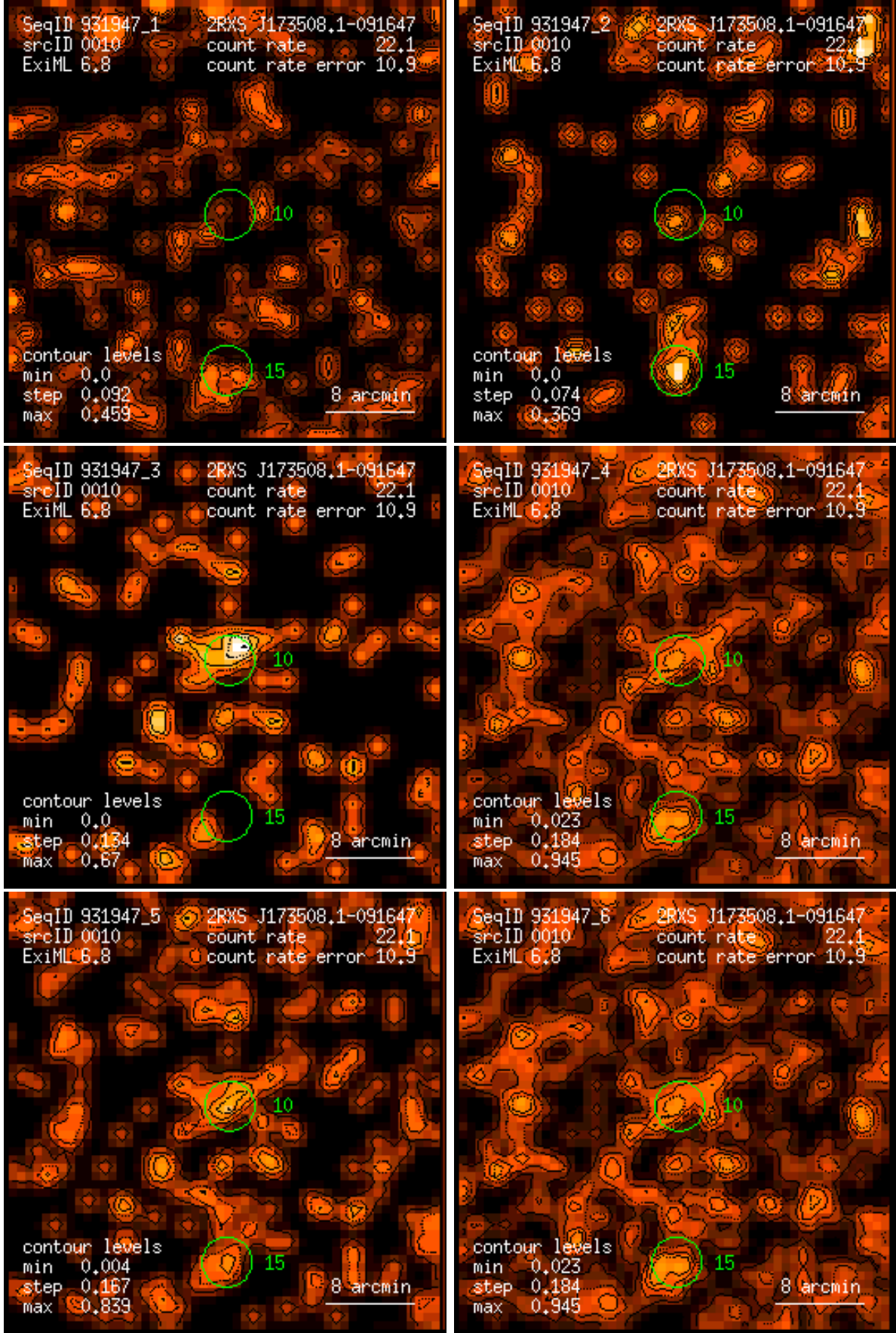
Figure 10: RASS 931947: detection 0010: band rate images, Gaussian filter: (1) PSPC channels 11 – 41, (2) 52 – 90, (3) 91 – 201, (4) 11 – 235, (5) 52 – 201, (6) 11 – 201. Broad band rates in counts/ks. Band rate contour levels in counts/ks/arcmin 2 .
