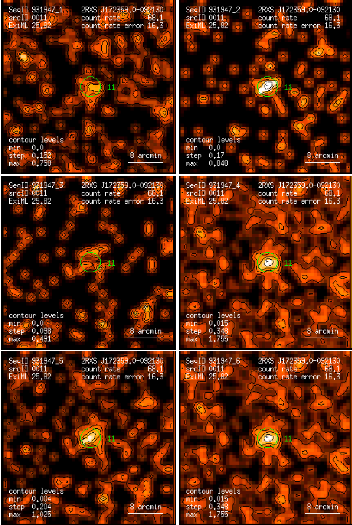
Figure 11: RASS 931947: detection 0011: band rate images, Gaussian filter: (1) PSPC channels 11 – 41, (2) 52 – 90, (3) 91 – 201, (4) 11 – 235, (5) 52 – 201, (6) 11 – 201. Broad band rates in counts/ks. Band rate contour levels in counts/ks/arcmin 2 .
