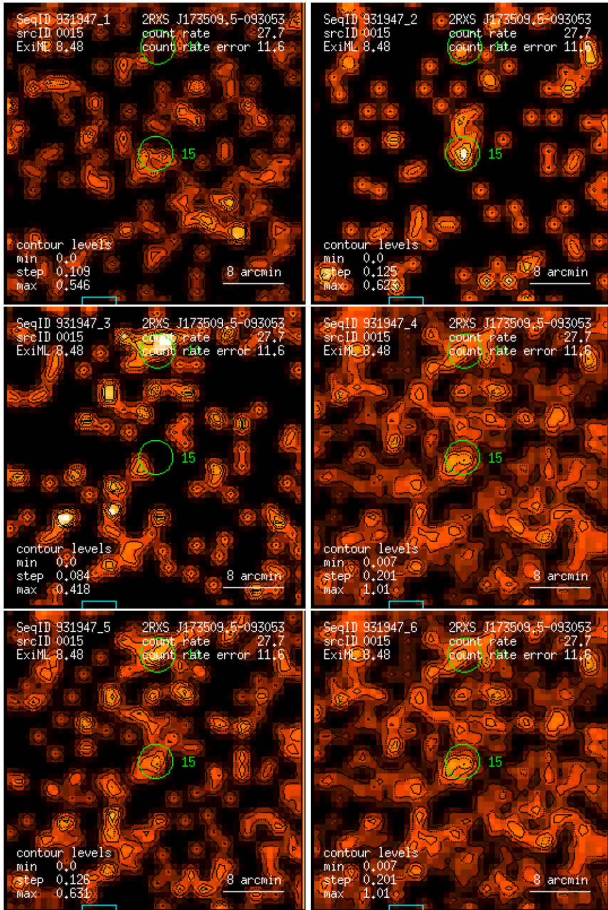
Figure 15: RASS 931947: detection 0015: band rate images, Gaussian filter: (1) PSPC channels 11 – 41, (2) 52 – 90, (3) 91 – 201, (4) 11 – 235, (5) 52 – 201, (6) 11 – 201. Broad band rates in counts/ks. Band rate contour levels in counts/ks/arcmin 2 .
