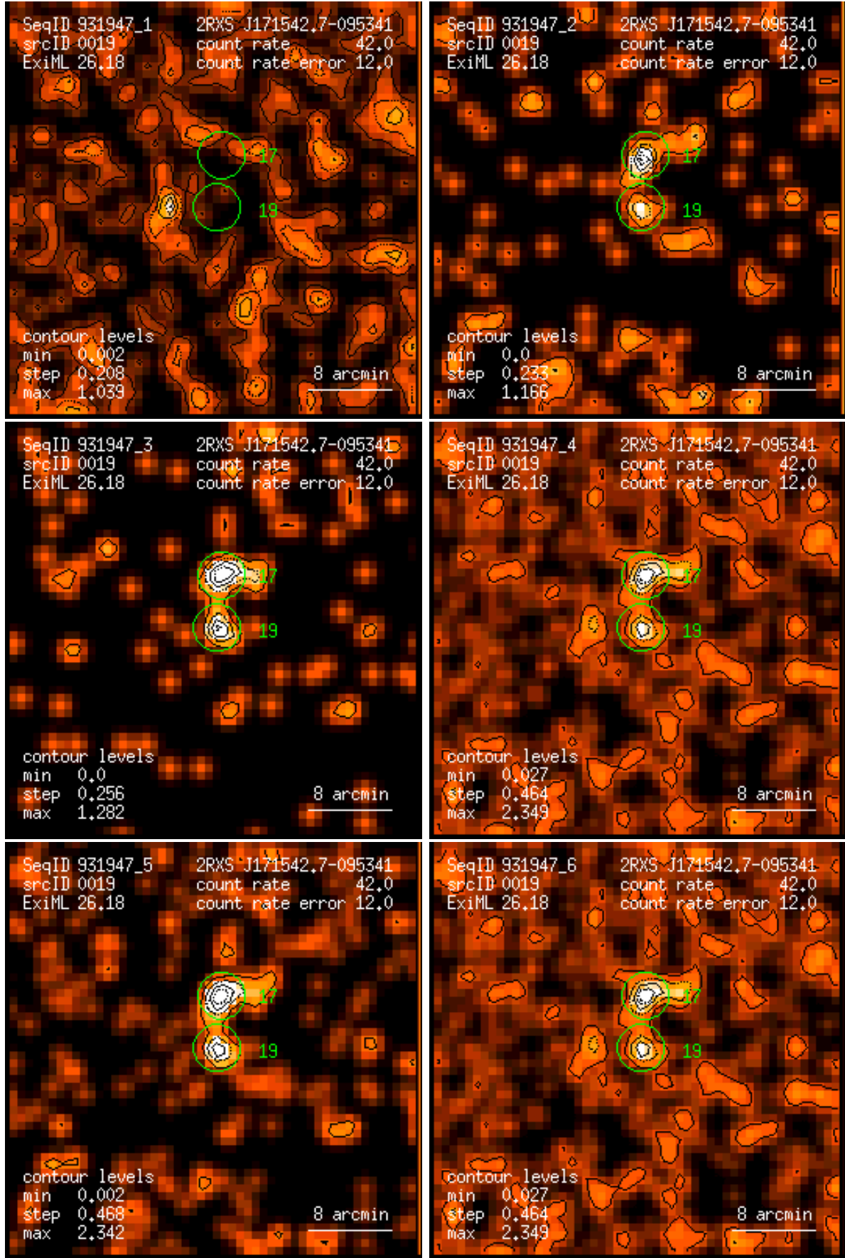
Figure 19: RASS 931947: detection 0019: band rate images, Gaussian filter: (1) PSPC channels 11 – 41, (2) 52 – 90, (3) 91 – 201, (4) 11 – 235, (5) 52 – 201, (6) 11 – 201. Broad band rates in counts/ks. Band rate contour levels in counts/ks/arcmin 2 .
