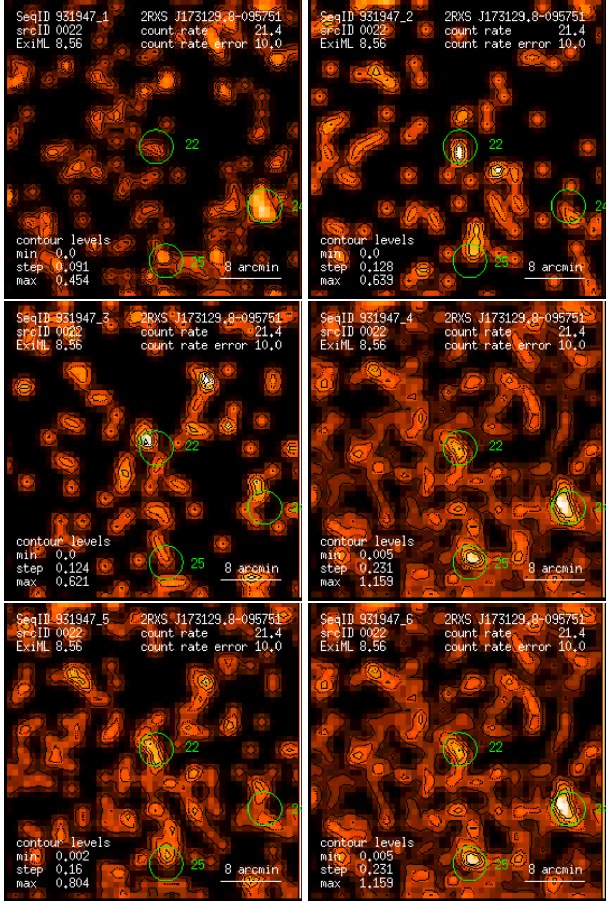
Figure 22: RASS 931947: detection 0022: band rate images, Gaussian filter: (1) PSPC channels 11 – 41, (2) 52 – 90, (3) 91 – 201, (4) 11 – 235, (5) 52 – 201, (6) 11 – 201. Broad band rates in counts/ks. Band rate contour levels in counts/ks/arcmin 2 .
