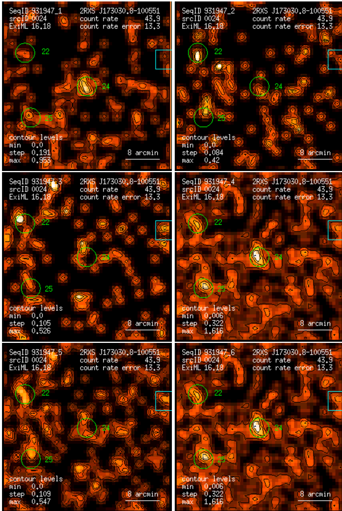
Figure 24: RASS 931947: detection 0024: band rate images, Gaussian filter: (1) PSPC channels 11 – 41, (2) 52 – 90, (3) 91 – 201, (4) 11 – 235, (5) 52 – 201, (6) 11 – 201. Broad band rates in counts/ks. Band rate contour levels in counts/ks/arcmin 2 .
