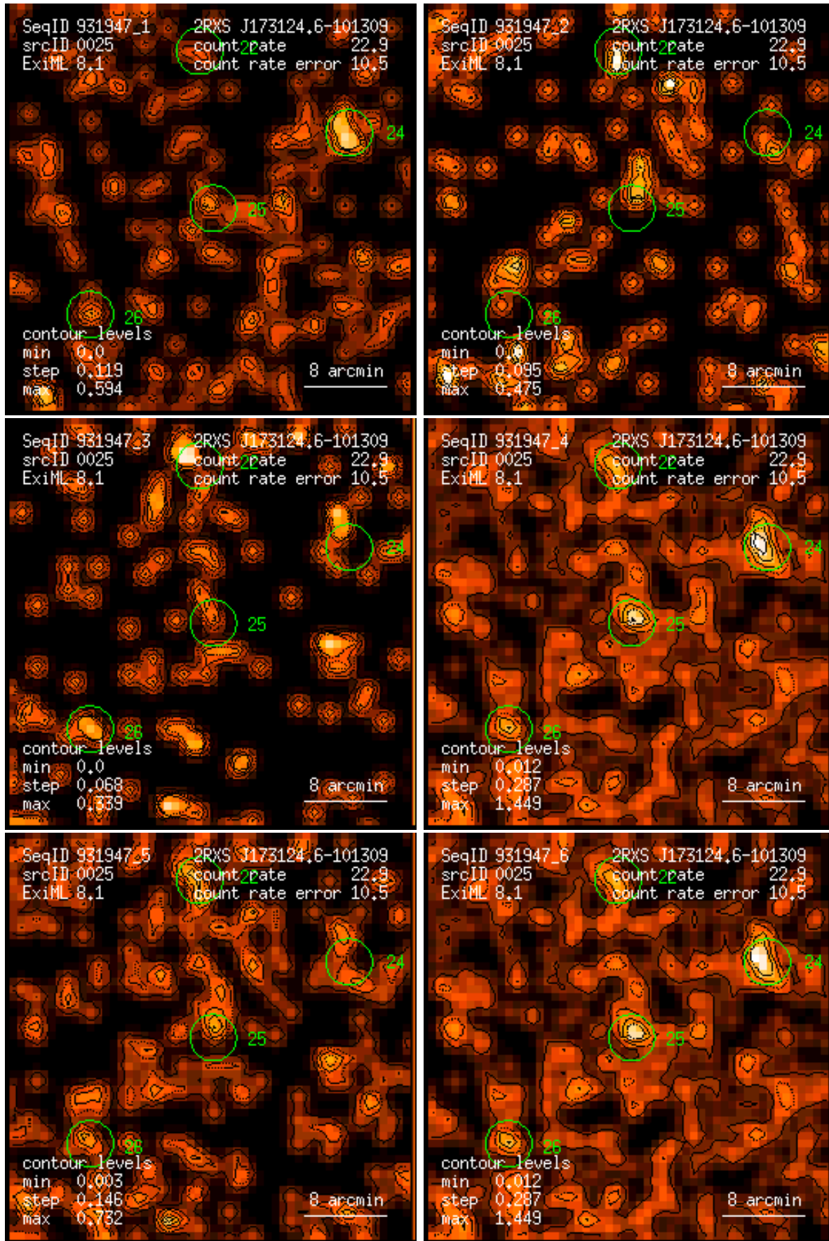
Figure 25: RASS 931947: detection 0025: band rate images, Gaussian filter: (1) PSPC channels 11 – 41, (2) 52 – 90, (3) 91 – 201, (4) 11 – 235, (5) 52 – 201, (6) 11 – 201. Broad band rates in counts/ks. Band rate contour levels in counts/ks/arcmin 2 .
