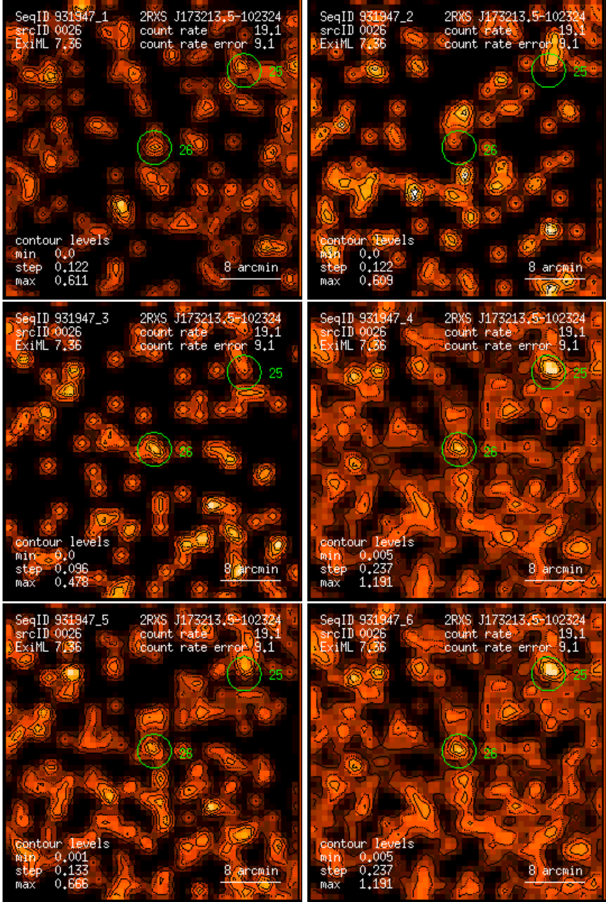
Figure 26: RASS 931947: detection 0026: band rate images, Gaussian filter: (1) PSPC channels 11 – 41, (2) 52 – 90, (3) 91 – 201, (4) 11 – 235, (5) 52 – 201, (6) 11 – 201. Broad band rates in counts/ks. Band rate contour levels in counts/ks/arcmin 2 .
