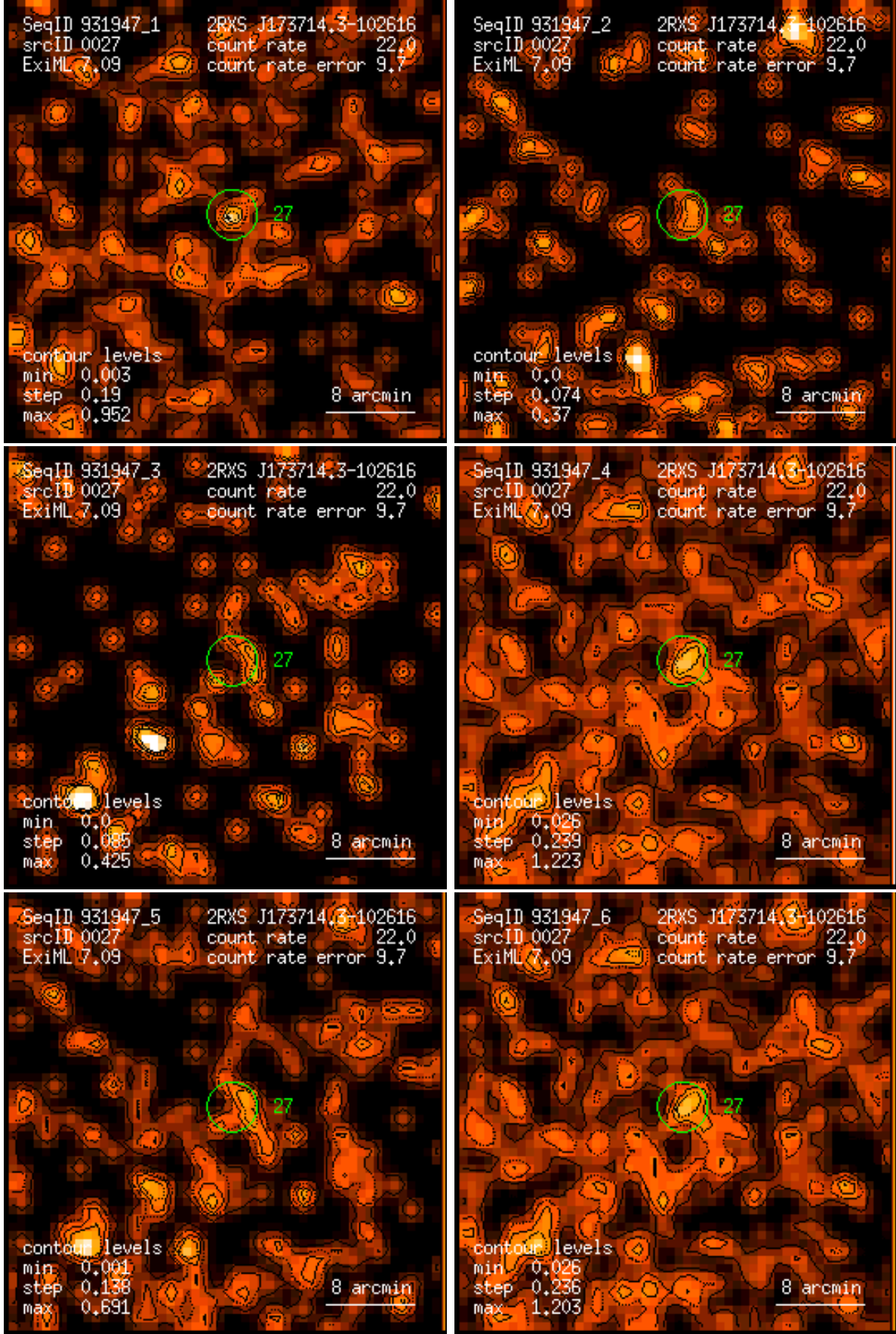
Figure 27: RASS 931947: detection 0027: band rate images, Gaussian filter: (1) PSPC channels 11 – 41, (2) 52 – 90, (3) 91 – 201, (4) 11 – 235, (5) 52 – 201, (6) 11 – 201. Broad band rates in counts/ks. Band rate contour levels in counts/ks/arcmin 2 .
