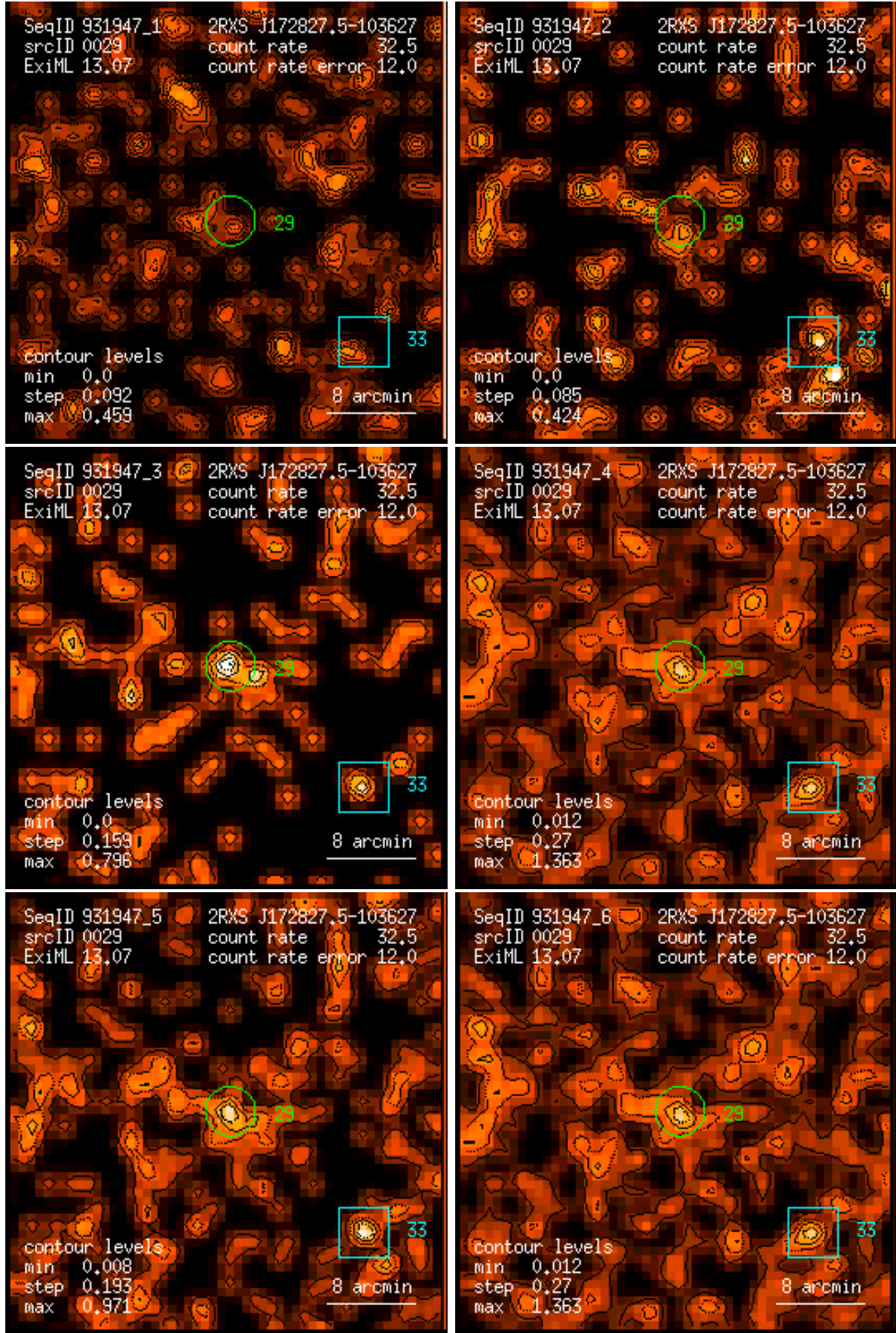
Figure 29: RASS 931947: detection 0029: band rate images, Gaussian filter: (1) PSPC channels 11 – 41, (2) 52 – 90, (3) 91 – 201, (4) 11 – 235, (5) 52 – 201, (6) 11 – 201. Broad band rates in counts/ks. Band rate contour levels in counts/ks/arcmin 2 .
