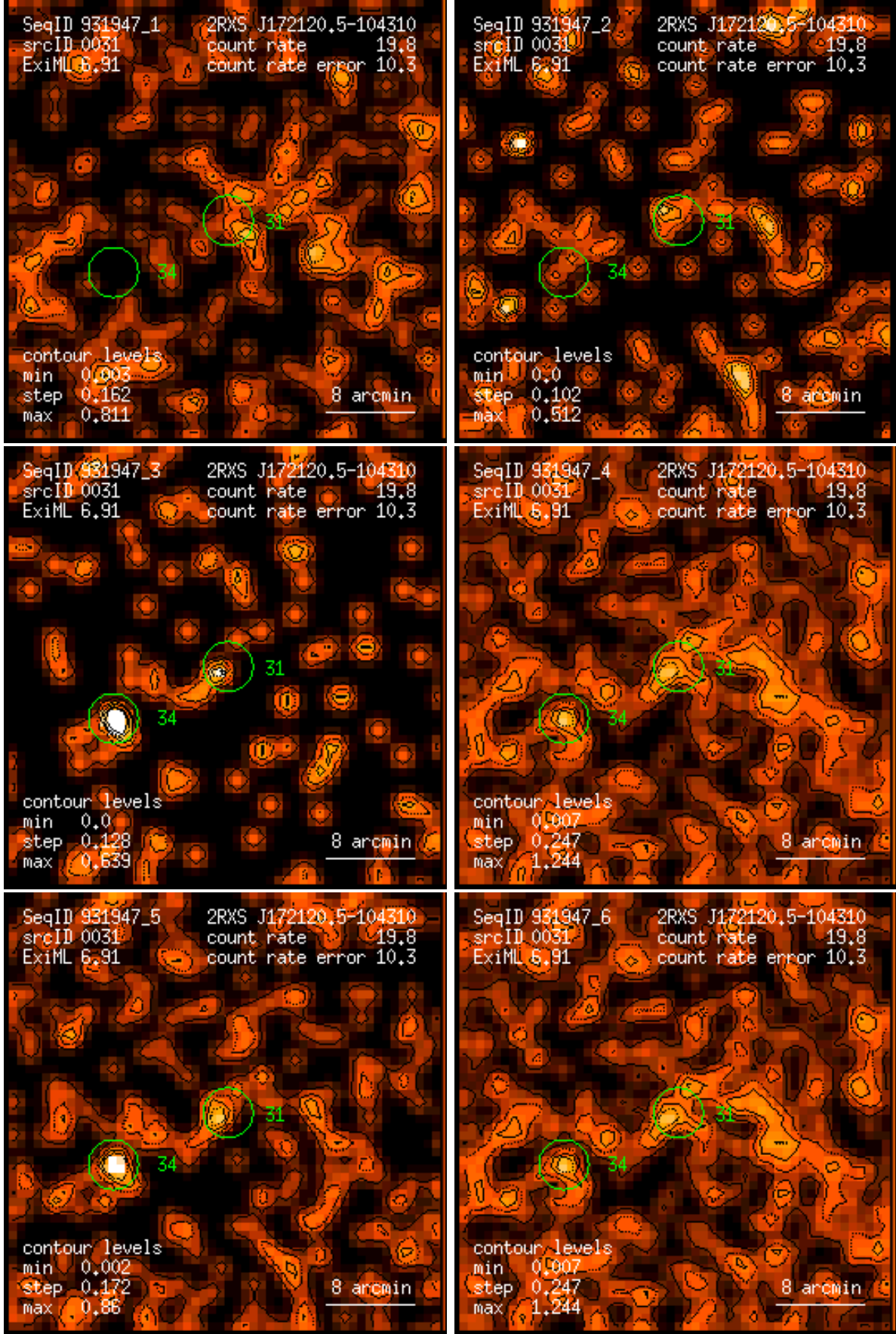
Figure 31: RASS 931947: detection 0031: band rate images, Gaussian filter: (1) PSPC channels 11 – 41, (2) 52 – 90, (3) 91 – 201, (4) 11 – 235, (5) 52 – 201, (6) 11 – 201. Broad band rates in counts/ks. Band rate contour levels in counts/ks/arcmin 2 .
