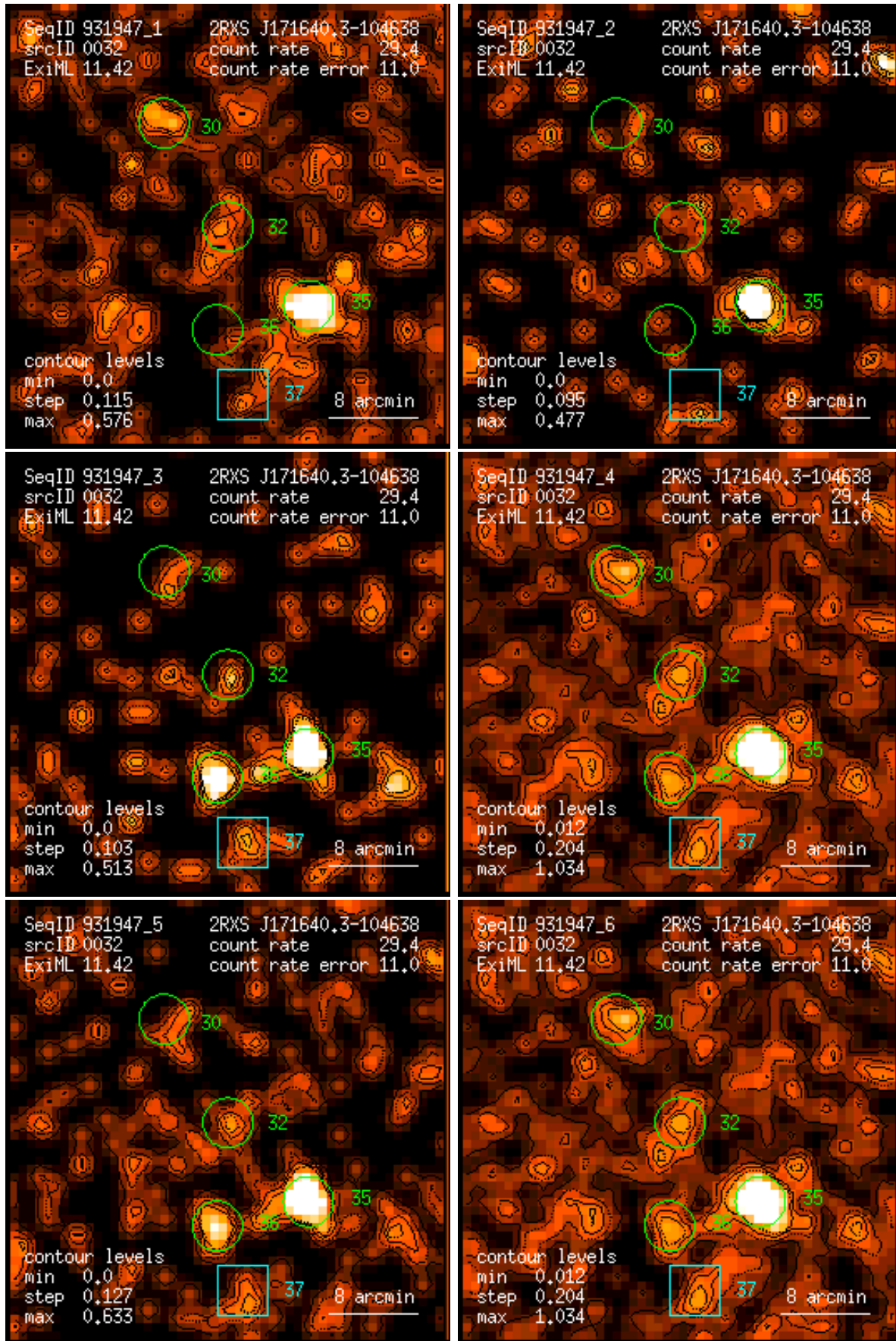
Figure 32: RASS 931947: detection 0032: band rate images, Gaussian filter: (1) PSPC channels 11 – 41, (2) 52 – 90, (3) 91 – 201, (4) 11 – 235, (5) 52 – 201, (6) 11 – 201. Broad band rates in counts/ks. Band rate contour levels in counts/ks/arcmin 2 .
