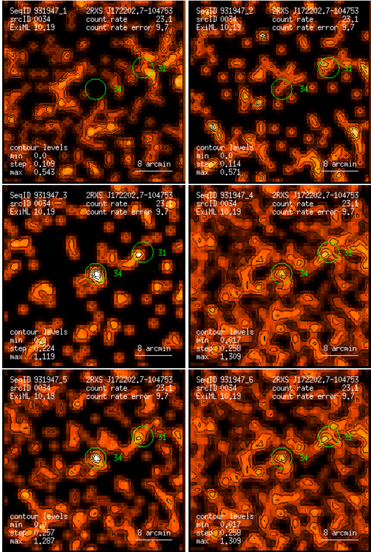
Figure 34: RASS 931947: detection 0034: band rate images, Gaussian filter: (1) PSPC channels 11 – 41, (2) 52 – 90, (3) 91 – 201, (4) 11 – 235, (5) 52 – 201, (6) 11 – 201. Broad band rates in counts/ks. Band rate contour levels in counts/ks/arcmin 2 .
