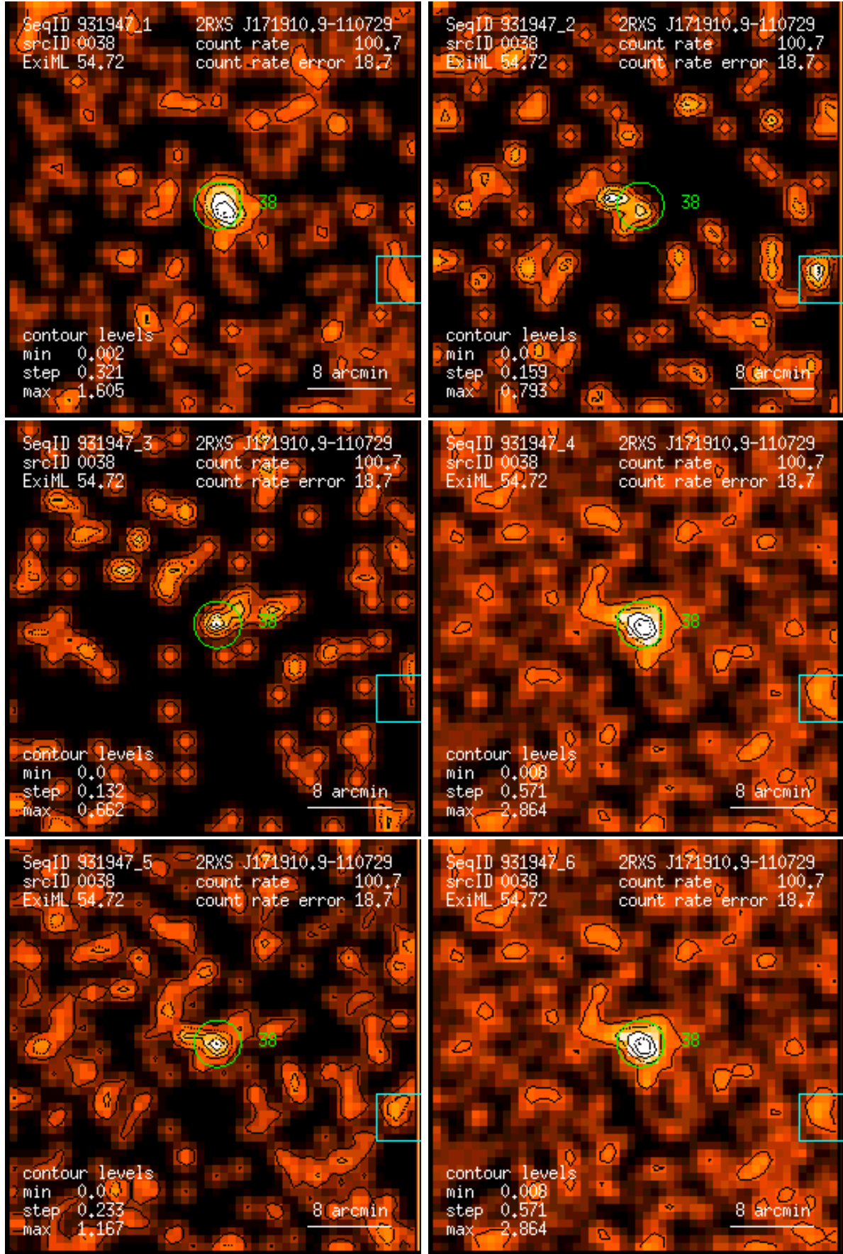
Figure 38: RASS 931947: detection 0038: band rate images, Gaussian filter: (1) PSPC channels 11 – 41, (2) 52 – 90, (3) 91 – 201, (4) 11 – 235, (5) 52 – 201, (6) 11 – 201. Broad band rates in counts/ks. Band rate contour levels in counts/ks/arcmin 2 .
