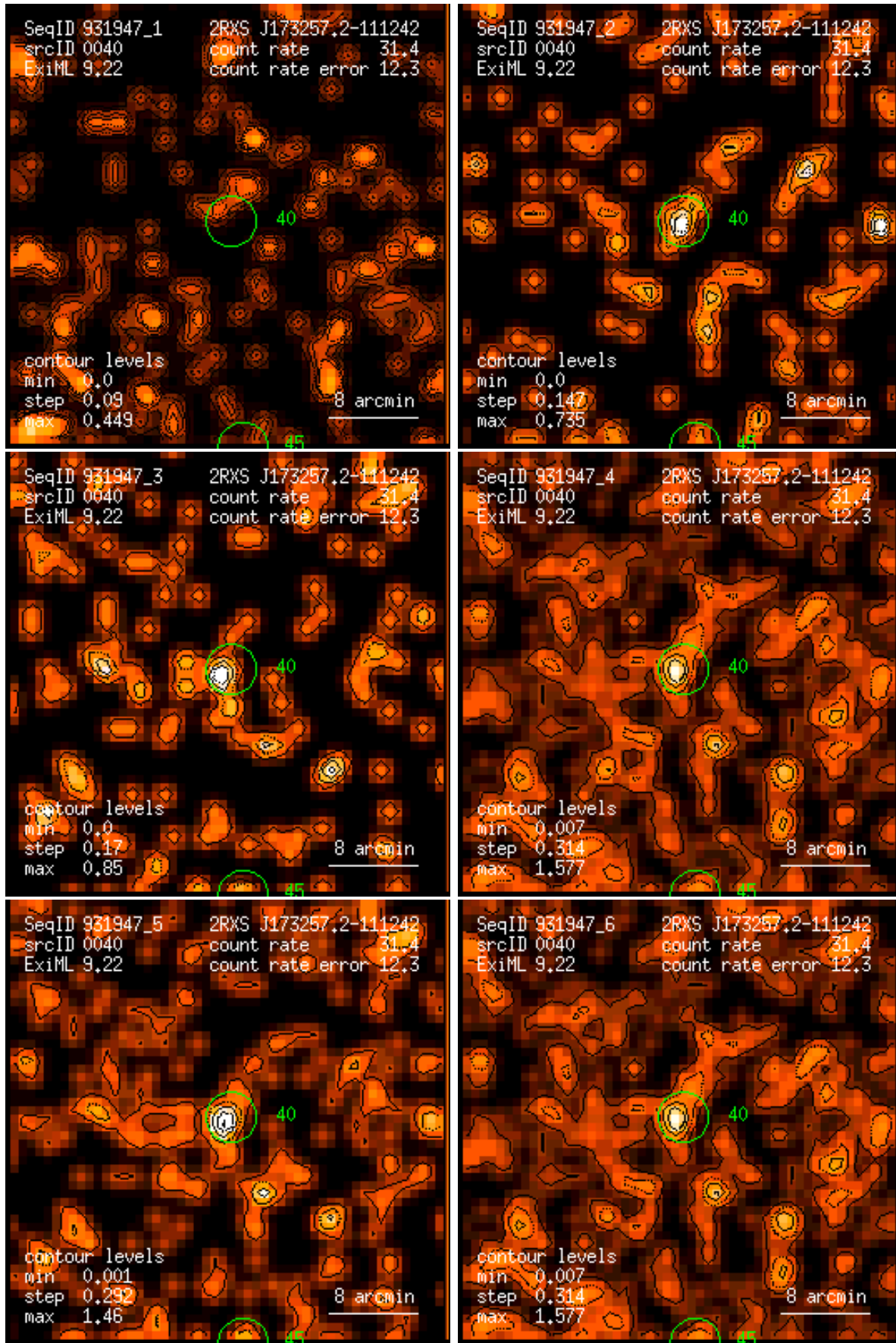
Figure 40: RASS 931947: detection 0040: band rate images, Gaussian filter: (1) PSPC channels 11 – 41, (2) 52 – 90, (3) 91 – 201, (4) 11 – 235, (5) 52 – 201, (6) 11 – 201. Broad band rates in counts/ks. Band rate contour levels in counts/ks/arcmin 2 .
