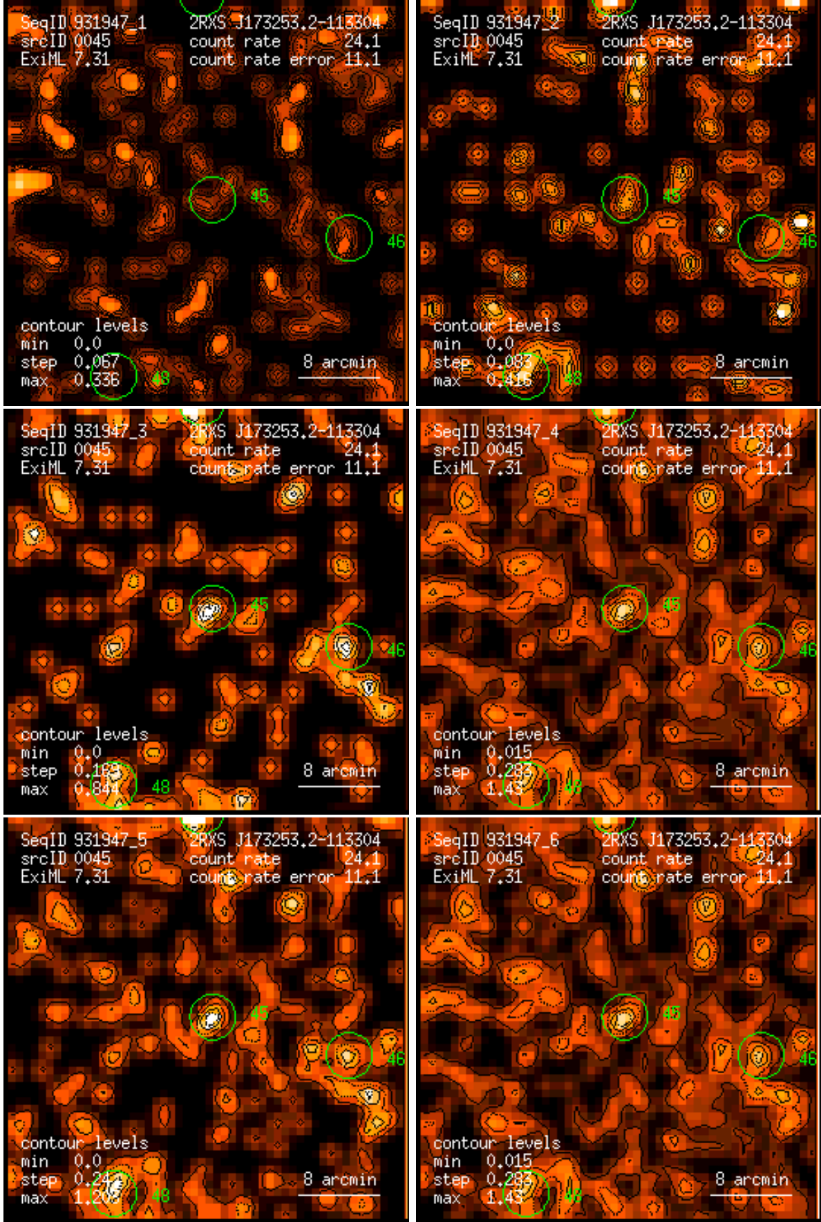
Figure 45: RASS 931947: detection 0045: band rate images, Gaussian filter: (1) PSPC channels 11 – 41, (2) 52 – 90, (3) 91 – 201, (4) 11 – 235, (5) 52 – 201, (6) 11 – 201. Broad band rates in counts/ks. Band rate contour levels in counts/ks/arcmin 2 .
