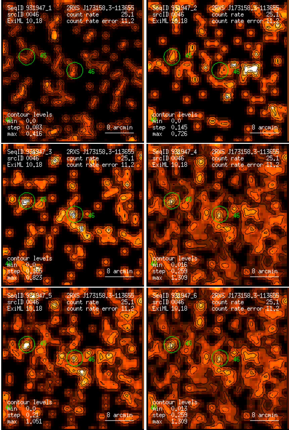
Figure 46: RASS 931947: detection 0046: band rate images, Gaussian filter: (1) PSPC channels 11 – 41, (2) 52 – 90, (3) 91 – 201, (4) 11 – 235, (5) 52 – 201, (6) 11 – 201. Broad band rates in counts/ks. Band rate contour levels in counts/ks/arcmin 2 .
