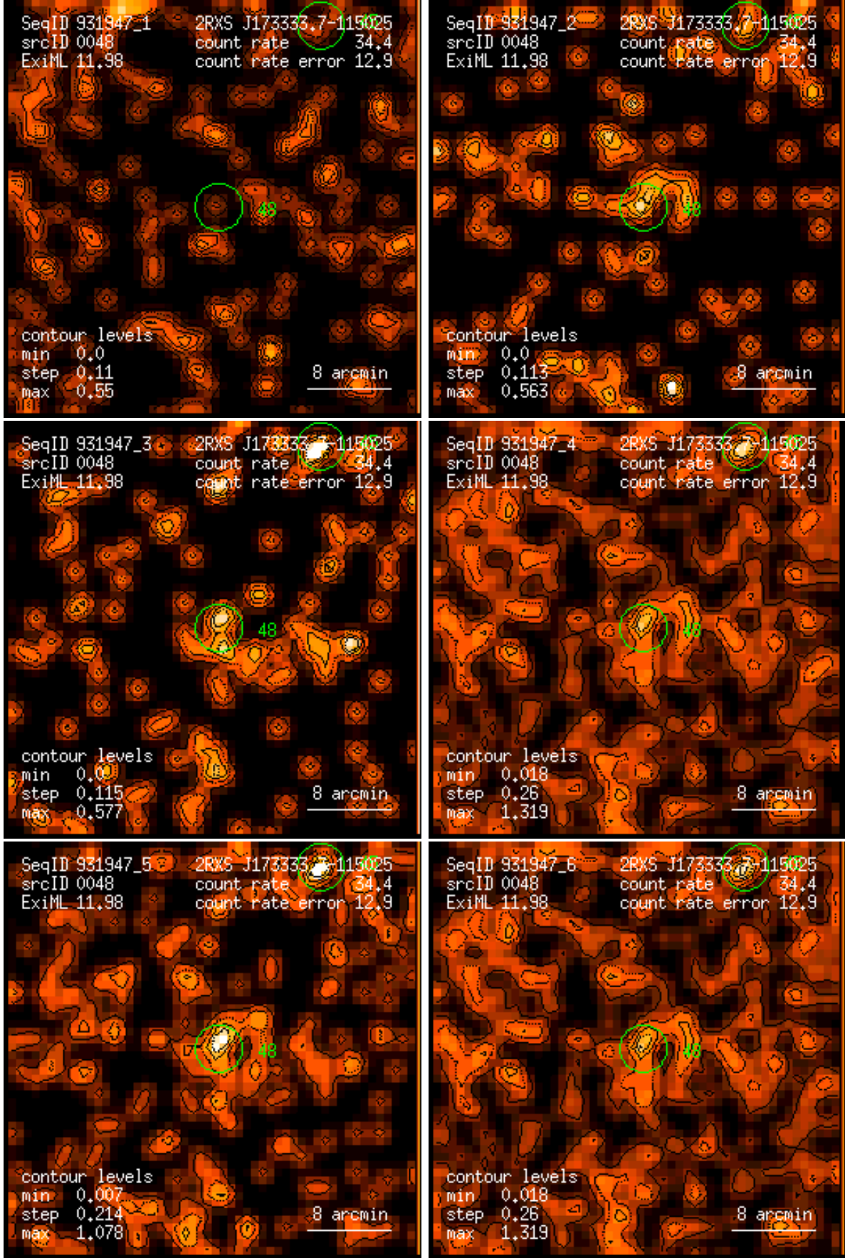
Figure 48: RASS 931947: detection 0048: band rate images, Gaussian filter: (1) PSPC channels 11 – 41, (2) 52 – 90, (3) 91 – 201, (4) 11 – 235, (5) 52 – 201, (6) 11 – 201. Broad band rates in counts/ks. Band rate contour levels in counts/ks/arcmin 2 .
