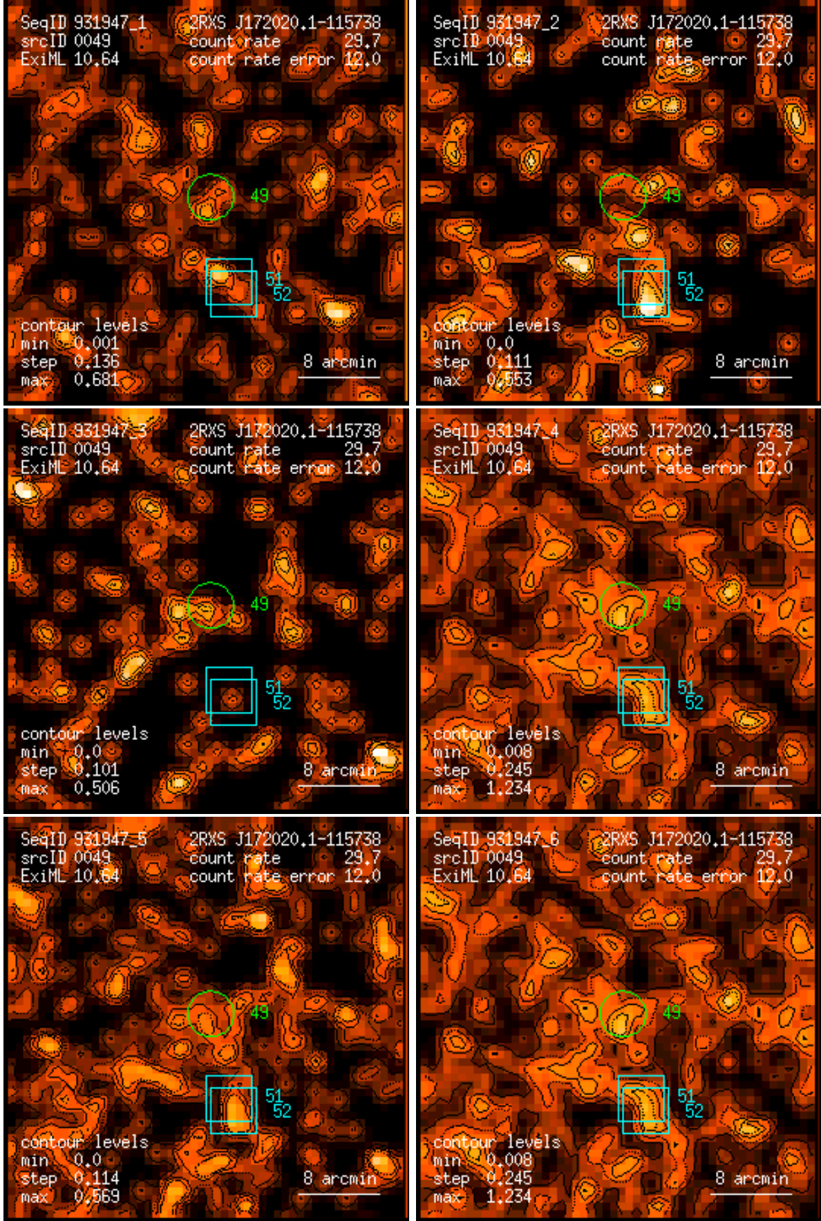
Figure 49: RASS 931947: detection 0049: band rate images, Gaussian filter: (1) PSPC channels 11 – 41, (2) 52 – 90, (3) 91 – 201, (4) 11 – 235, (5) 52 – 201, (6) 11 – 201. Broad band rates in counts/ks. Band rate contour levels in counts/ks/arcmin 2 .
