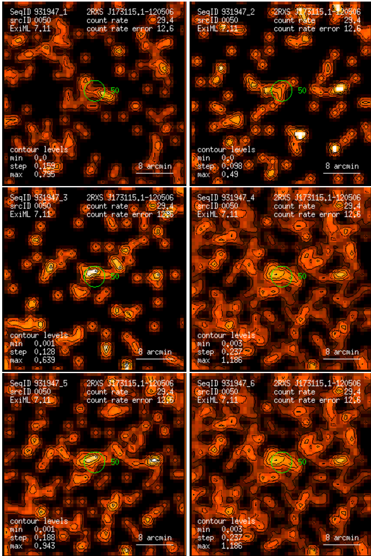
Figure 50: RASS 931947: detection 0050: band rate images, Gaussian filter: (1) PSPC channels 11 – 41, (2) 52 – 90, (3) 91 – 201, (4) 11 – 235, (5) 52 – 201, (6) 11 – 201. Broad band rates in counts/ks. Band rate contour levels in counts/ks/arcmin 2 .
