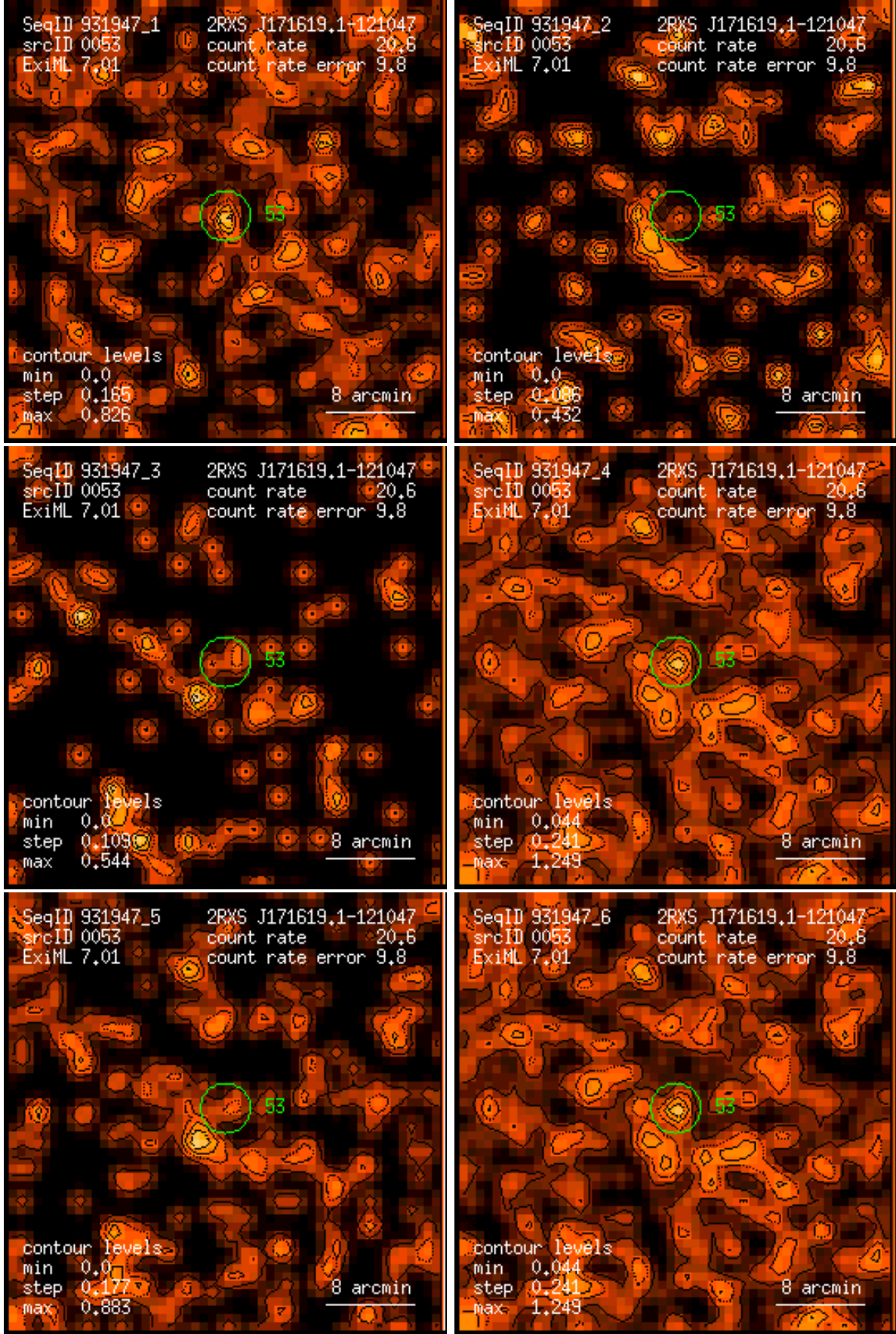
Figure 53: RASS 931947: detection 0053: band rate images, Gaussian filter: (1) PSPC channels 11 – 41, (2) 52 – 90, (3) 91 – 201, (4) 11 – 235, (5) 52 – 201, (6) 11 – 201. Broad band rates in counts/ks. Band rate contour levels in counts/ks/arcmin 2 .
