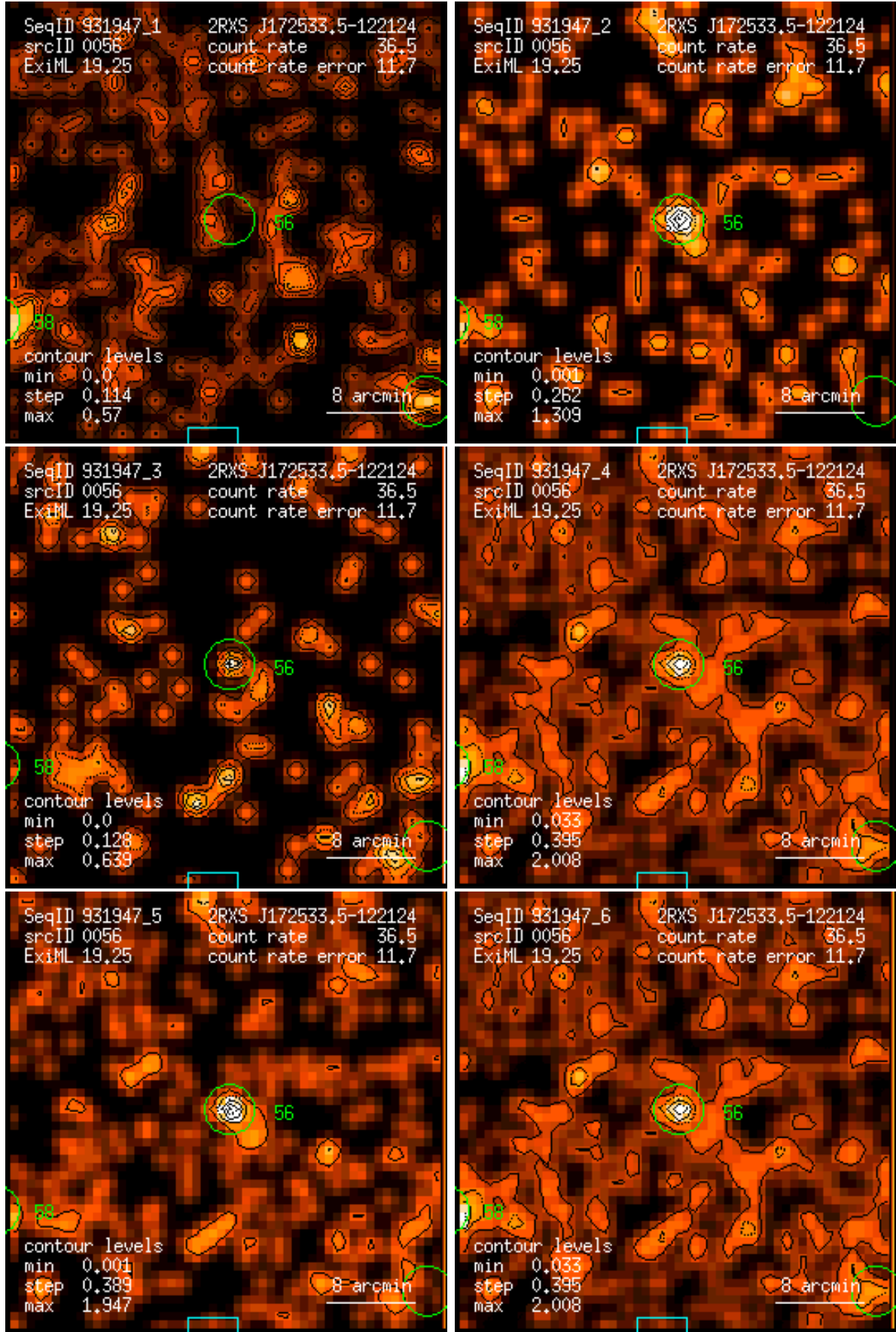
Figure 56: RASS 931947: detection 0056: band rate images, Gaussian filter: (1) PSPC channels 11 – 41, (2) 52 – 90, (3) 91 – 201, (4) 11 – 235, (5) 52 – 201, (6) 11 – 201. Broad band rates in counts/ks. Band rate contour levels in counts/ks/arcmin 2 .
