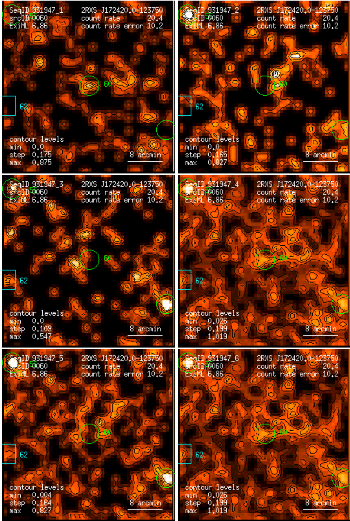
Figure 60: RASS 931947: detection 0060: band rate images, Gaussian filter: (1) PSPC channels 11 – 41, (2) 52 – 90, (3) 91 – 201, (4) 11 – 235, (5) 52 – 201, (6) 11 – 201. Broad band rates in counts/ks. Band rate contour levels in counts/ks/arcmin 2 .
