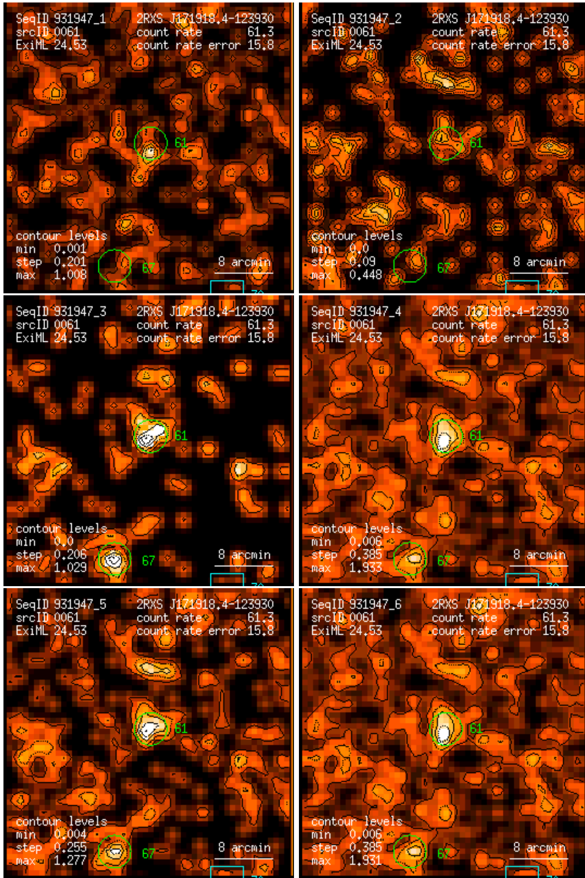
Figure 61: RASS 931947: detection 0061: band rate images, Gaussian filter: (1) PSPC channels 11 – 41, (2) 52 – 90, (3) 91 – 201, (4) 11 – 235, (5) 52 – 201, (6) 11 – 201. Broad band rates in counts/ks. Band rate contour levels in counts/ks/arcmin 2 .
