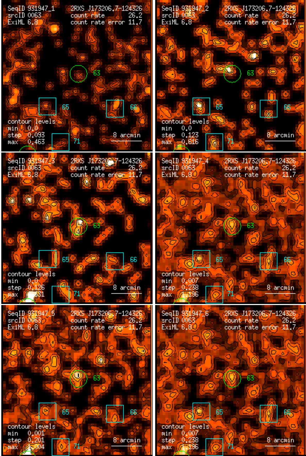
Figure 63: RASS 931947: detection 0063: band rate images, Gaussian filter: (1) PSPC channels 11 – 41, (2) 52 – 90, (3) 91 – 201, (4) 11 – 235, (5) 52 – 201, (6) 11 – 201. Broad band rates in counts/ks. Band rate contour levels in counts/ks/arcmin 2 .
