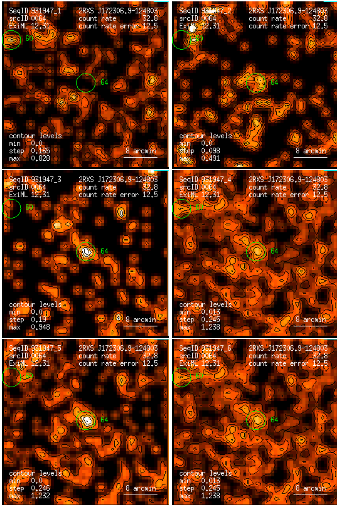
Figure 64: RASS 931947: detection 0064: band rate images, Gaussian filter: (1) PSPC channels 11 – 41, (2) 52 – 90, (3) 91 – 201, (4) 11 – 235, (5) 52 – 201, (6) 11 – 201. Broad band rates in counts/ks. Band rate contour levels in counts/ks/arcmin 2 .
