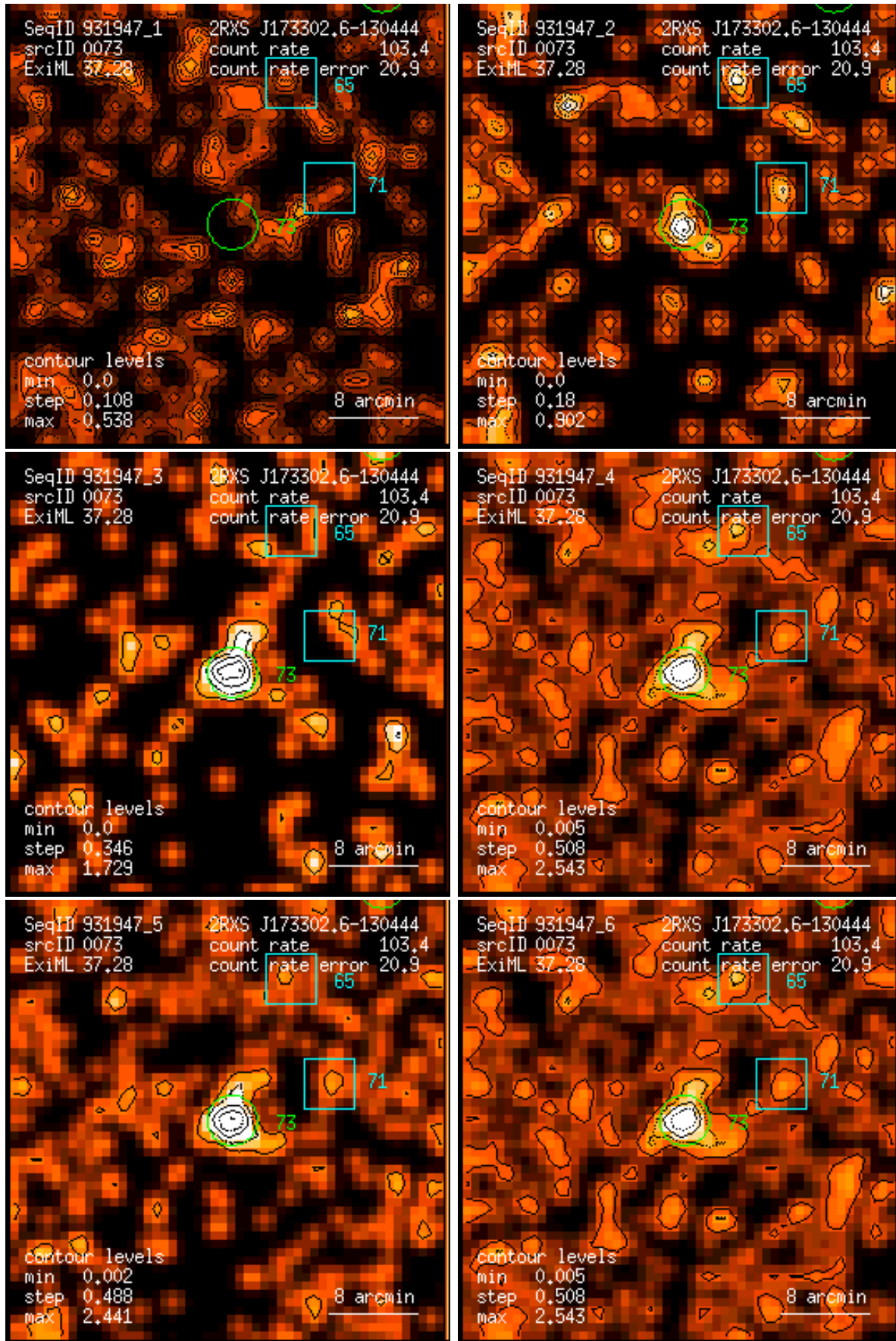
Figure 73: RASS 931947: detection 0073: band rate images, Gaussian filter: (1) PSPC channels 11 – 41, (2) 52 – 90, (3) 91 – 201, (4) 11 – 235, (5) 52 – 201, (6) 11 – 201. Broad band rates in counts/ks. Band rate contour levels in counts/ks/arcmin 2 .
