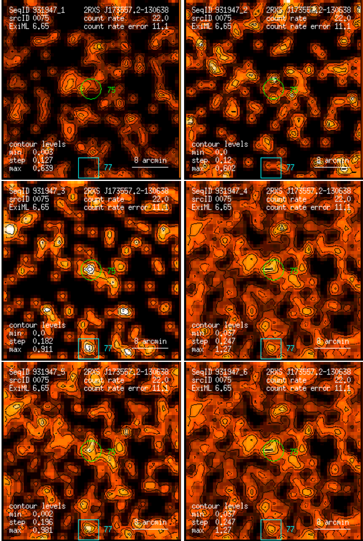
Figure 75: RASS 931947: detection 0075: band rate images, Gaussian filter: (1) PSPC channels 11 – 41, (2) 52 – 90, (3) 91 – 201, (4) 11 – 235, (5) 52 – 201, (6) 11 – 201. Broad band rates in counts/ks. Band rate contour levels in counts/ks/arcmin 2 .
