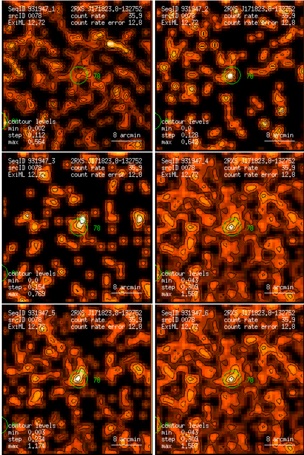
Figure 78: RASS 931947: detection 0078: band rate images, Gaussian filter: (1) PSPC channels 11 – 41, (2) 52 – 90, (3) 91 – 201, (4) 11 – 235, (5) 52 – 201, (6) 11 – 201. Broad band rates in counts/ks. Band rate contour levels in counts/ks/arcmin 2 .
