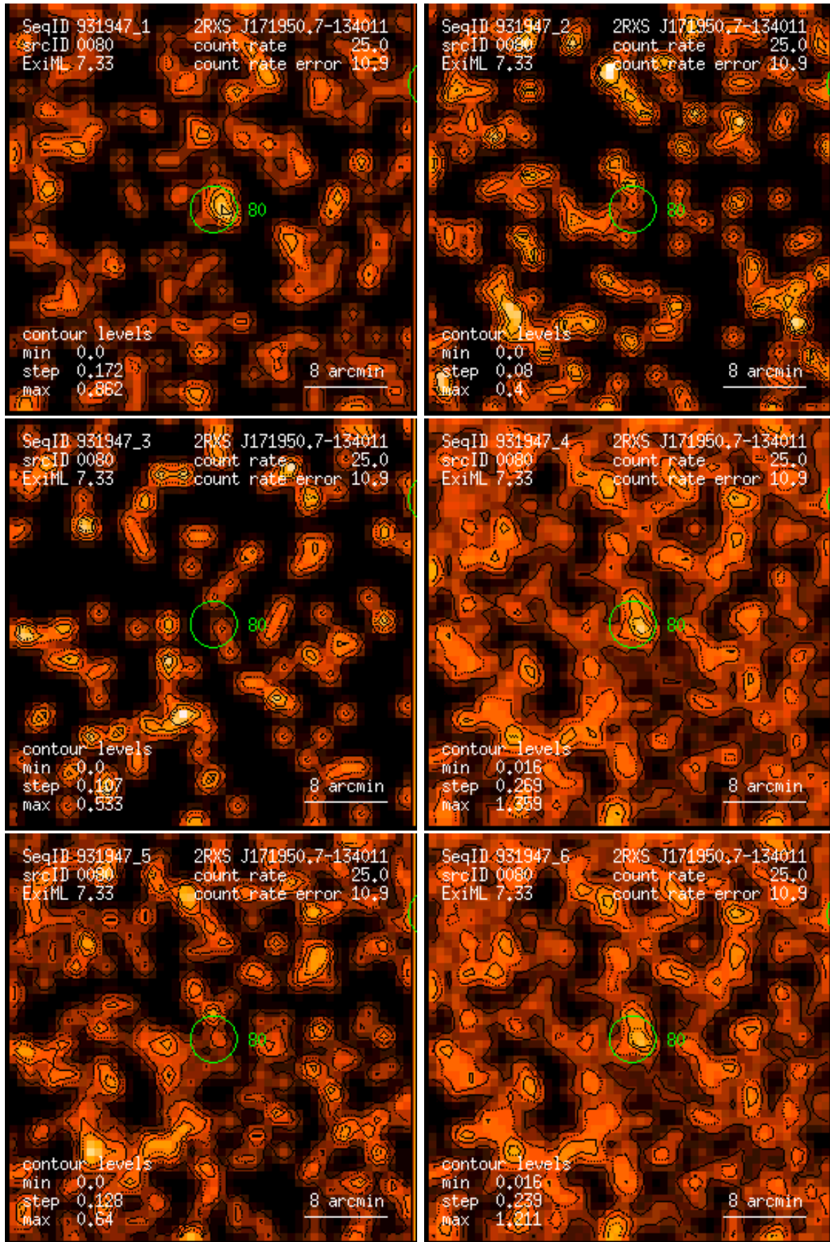
Figure 80: RASS 931947: detection 0080: band rate images, Gaussian filter: (1) PSPC channels 11 – 41, (2) 52 – 90, (3) 91 – 201, (4) 11 – 235, (5) 52 – 201, (6) 11 – 201. Broad band rates in counts/ks. Band rate contour levels in counts/ks/arcmin 2 .
