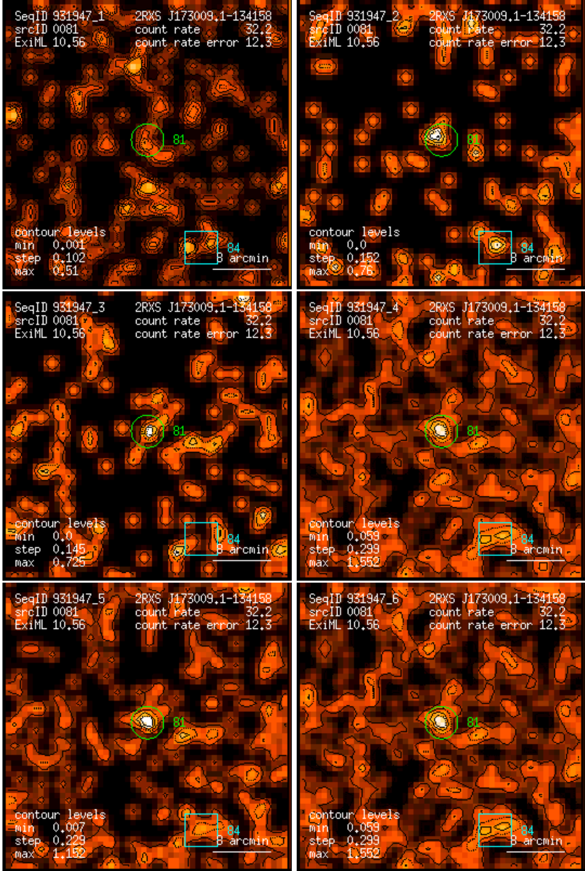
Figure 81: RASS 931947: detection 0081: band rate images, Gaussian filter: (1) PSPC channels 11 – 41, (2) 52 – 90, (3) 91 – 201, (4) 11 – 235, (5) 52 – 201, (6) 11 – 201. Broad band rates in counts/ks. Band rate contour levels in counts/ks/arcmin 2 .
