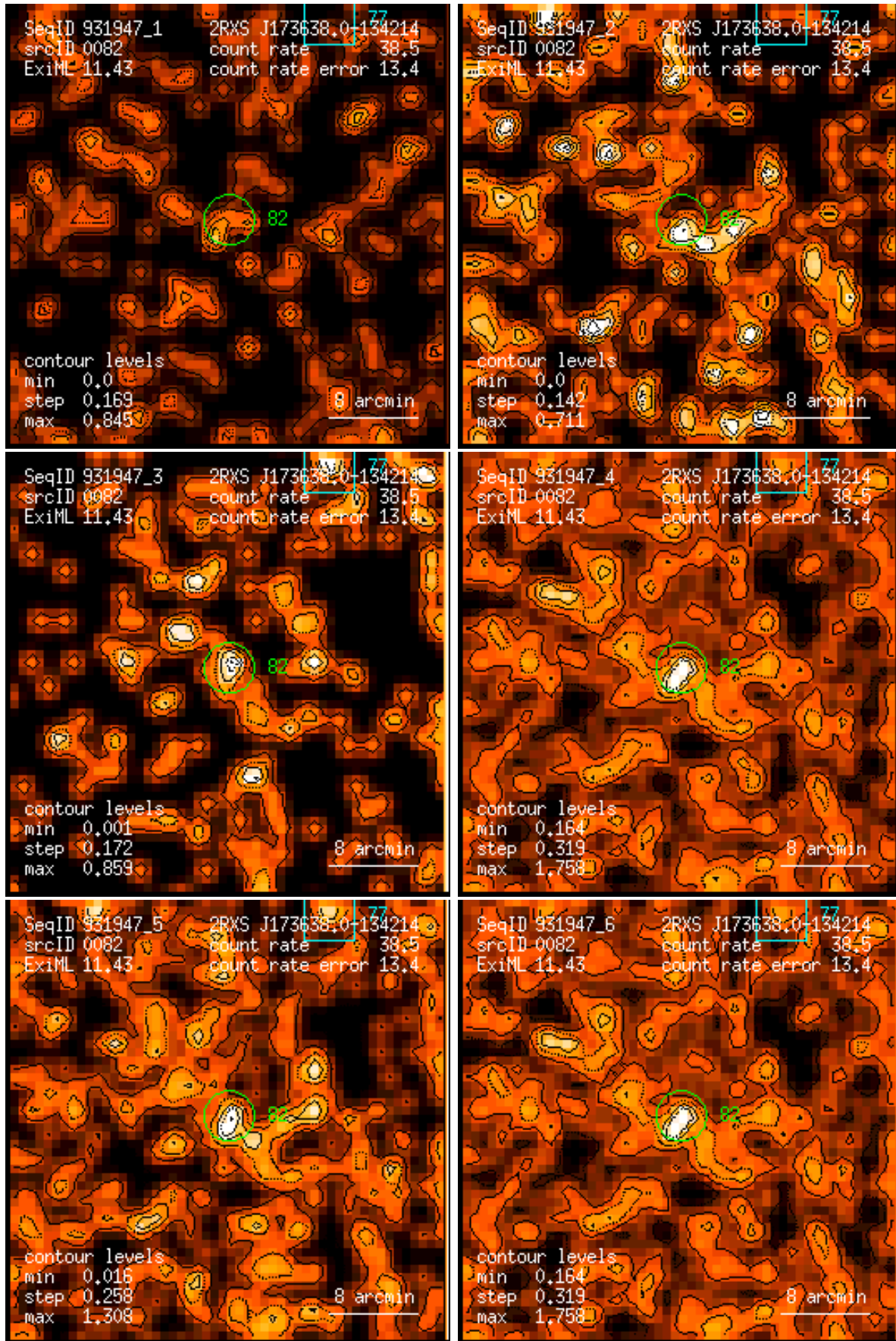
Figure 82: RASS 931947: detection 0082: band rate images, Gaussian filter: (1) PSPC channels 11 – 41, (2) 52 – 90, (3) 91 – 201, (4) 11 – 235, (5) 52 – 201, (6) 11 – 201. Broad band rates in counts/ks. Band rate contour levels in counts/ks/arcmin 2 .
