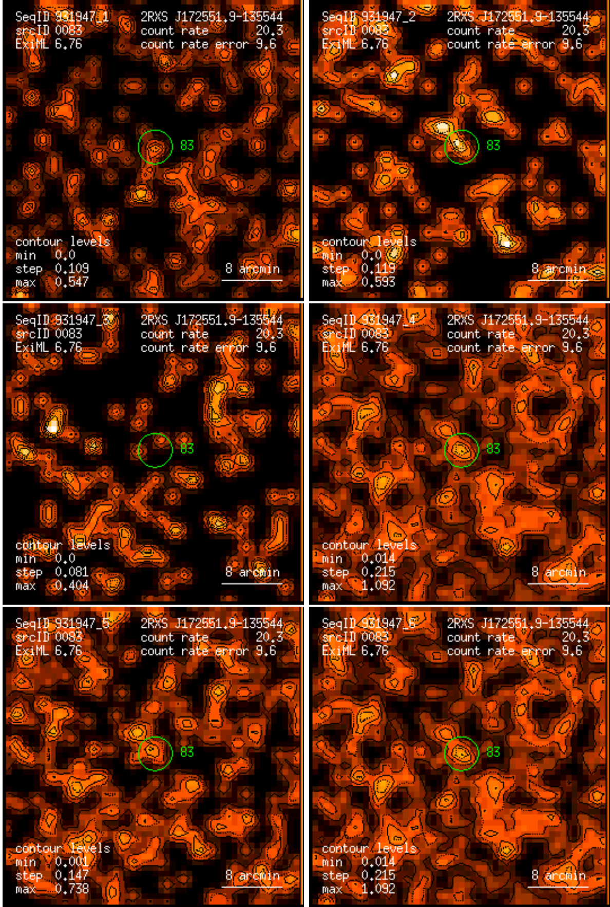
Figure 83: RASS 931947: detection 0083: band rate images, Gaussian filter: (1) PSPC channels 11 – 41, (2) 52 – 90, (3) 91 – 201, (4) 11 – 235, (5) 52 – 201, (6) 11 – 201. Broad band rates in counts/ks. Band rate contour levels in counts/ks/arcmin 2 .
