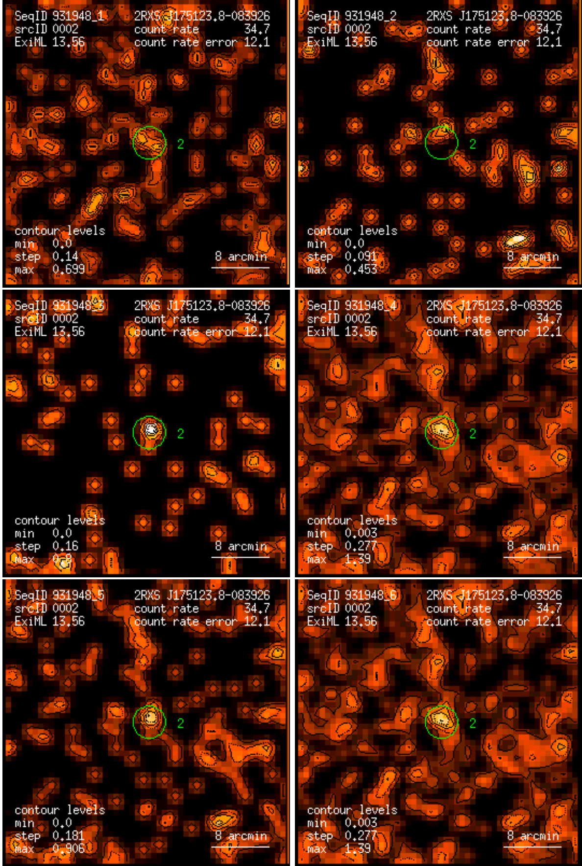
Figure 2: RASS 931948: detection 0002: band rate images, Gaussian filter: (1) PSPC channels 11 – 41, (2) 52 – 90, (3) 91 – 201, (4) 11 – 235, (5) 52 – 201, (6) 11 – 201. Broad band rates in counts/ks. Band rate contour levels in counts/ks/arcmin 2 .
