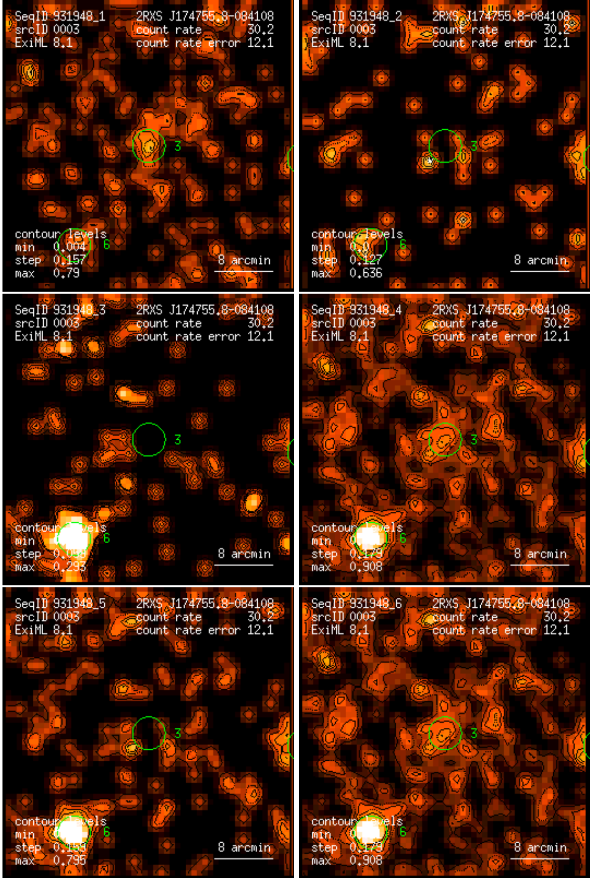
Figure 3: RASS 931948: detection 0003: band rate images, Gaussian filter: (1) PSPC channels 11 – 41, (2) 52 – 90, (3) 91 – 201, (4) 11 – 235, (5) 52 – 201, (6) 11 – 201. Broad band rates in counts/ks. Band rate contour levels in counts/ks/arcmin 2 .
