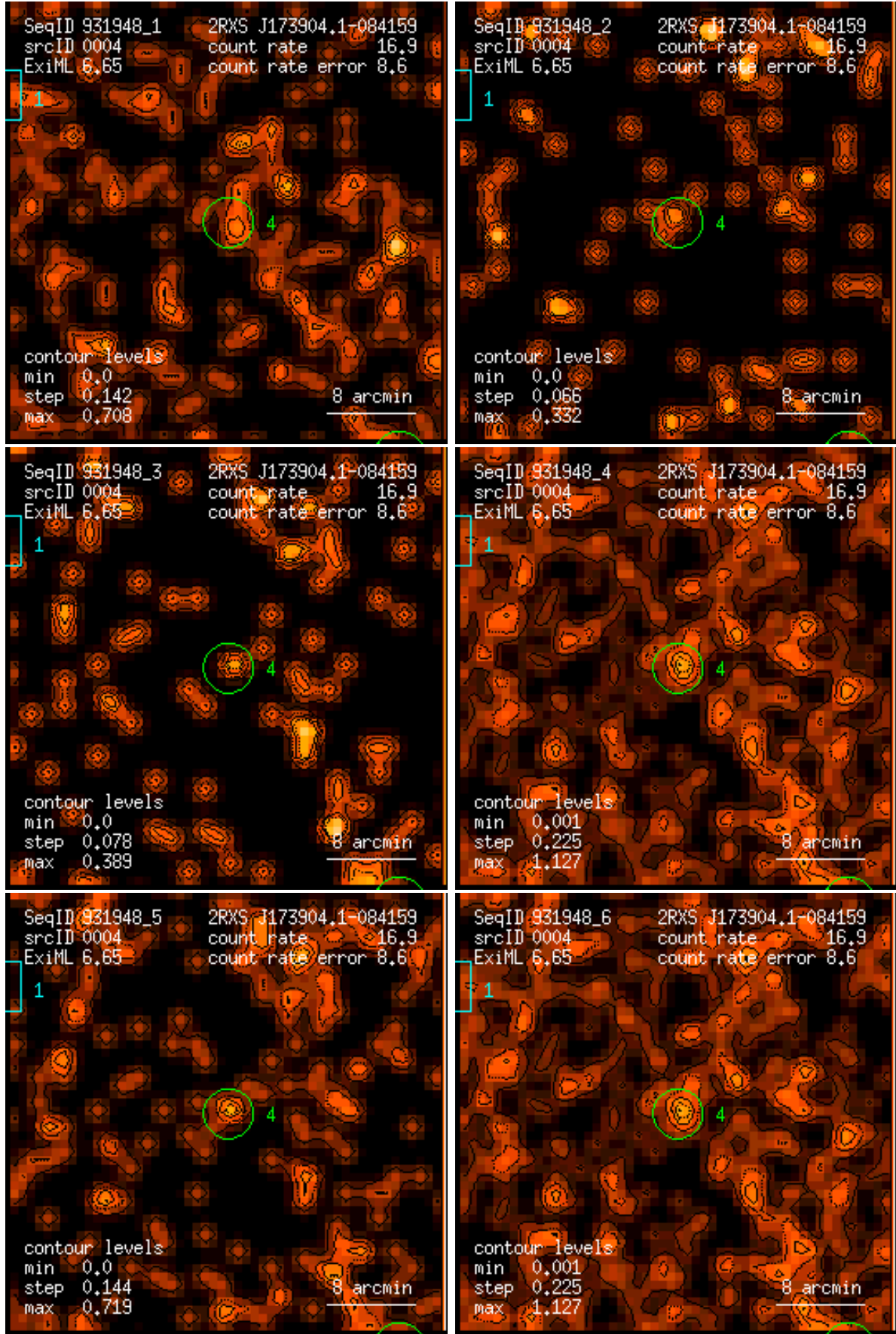
Figure 4: RASS 931948: detection 0004: band rate images, Gaussian filter: (1) PSPC channels 11 – 41, (2) 52 – 90, (3) 91 – 201, (4) 11 – 235, (5) 52 – 201, (6) 11 – 201. Broad band rates in counts/ks. Band rate contour levels in counts/ks/arcmin 2 .
