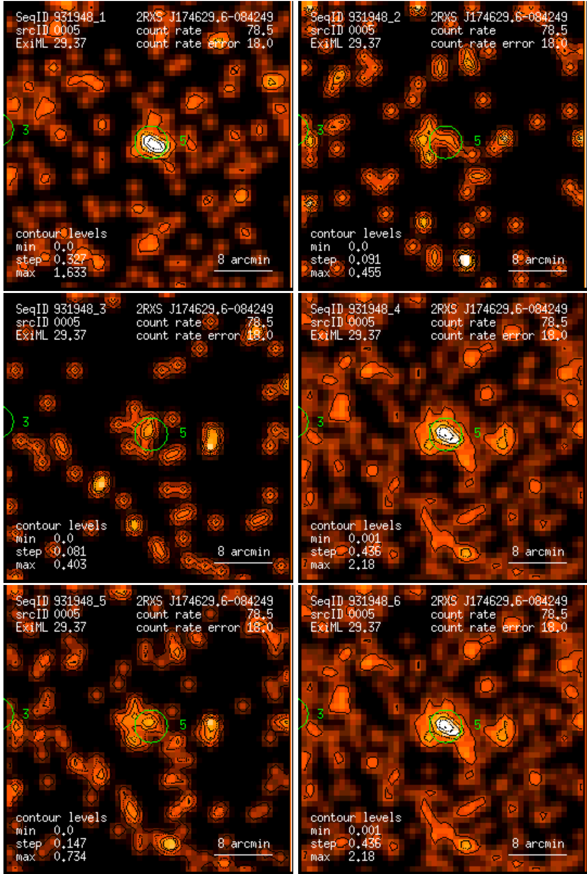
Figure 5: RASS 931948: detection 0005: band rate images, Gaussian filter: (1) PSPC channels 11 – 41, (2) 52 – 90, (3) 91 – 201, (4) 11 – 235, (5) 52 – 201, (6) 11 – 201. Broad band rates in counts/ks. Band rate contour levels in counts/ks/arcmin 2 .
