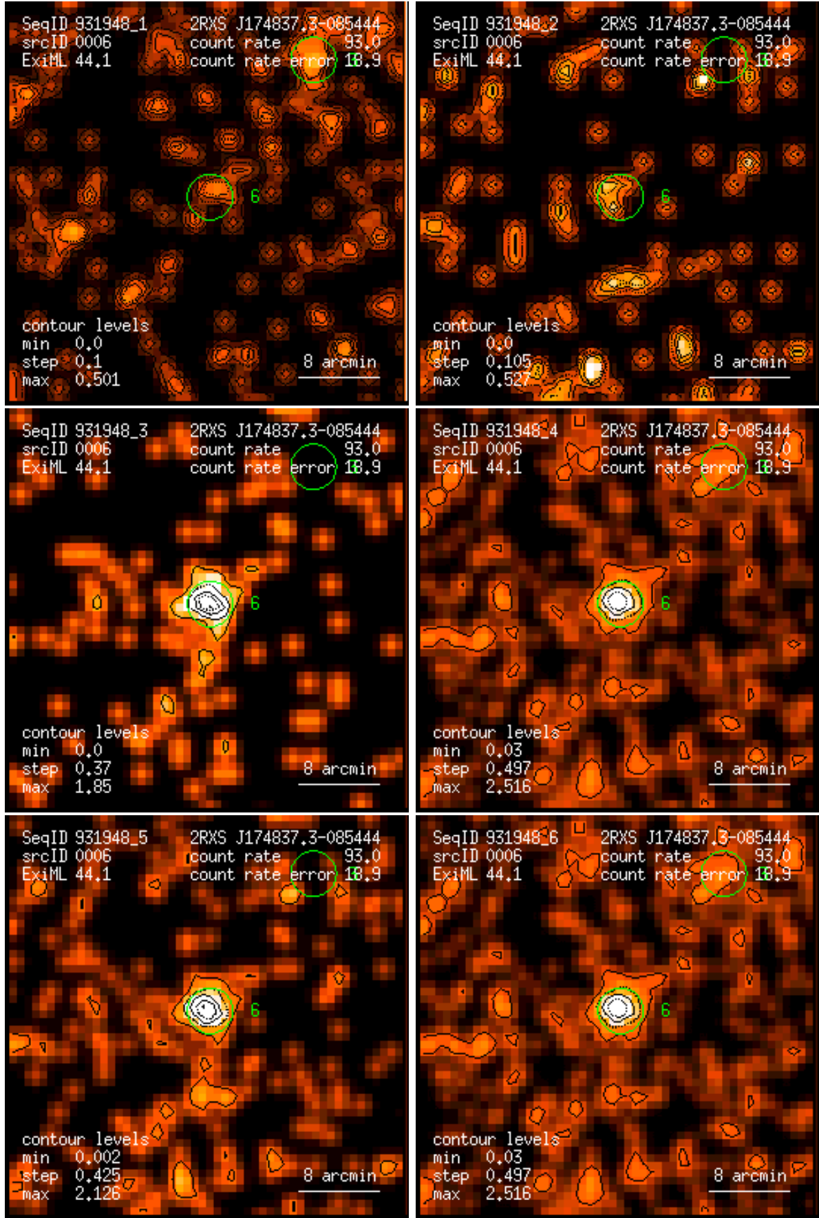
Figure 6: RASS 931948: detection 0006: band rate images, Gaussian filter: (1) PSPC channels 11 – 41, (2) 52 – 90, (3) 91 – 201, (4) 11 – 235, (5) 52 – 201, (6) 11 – 201. Broad band rates in counts/ks. Band rate contour levels in counts/ks/arcmin 2 .
