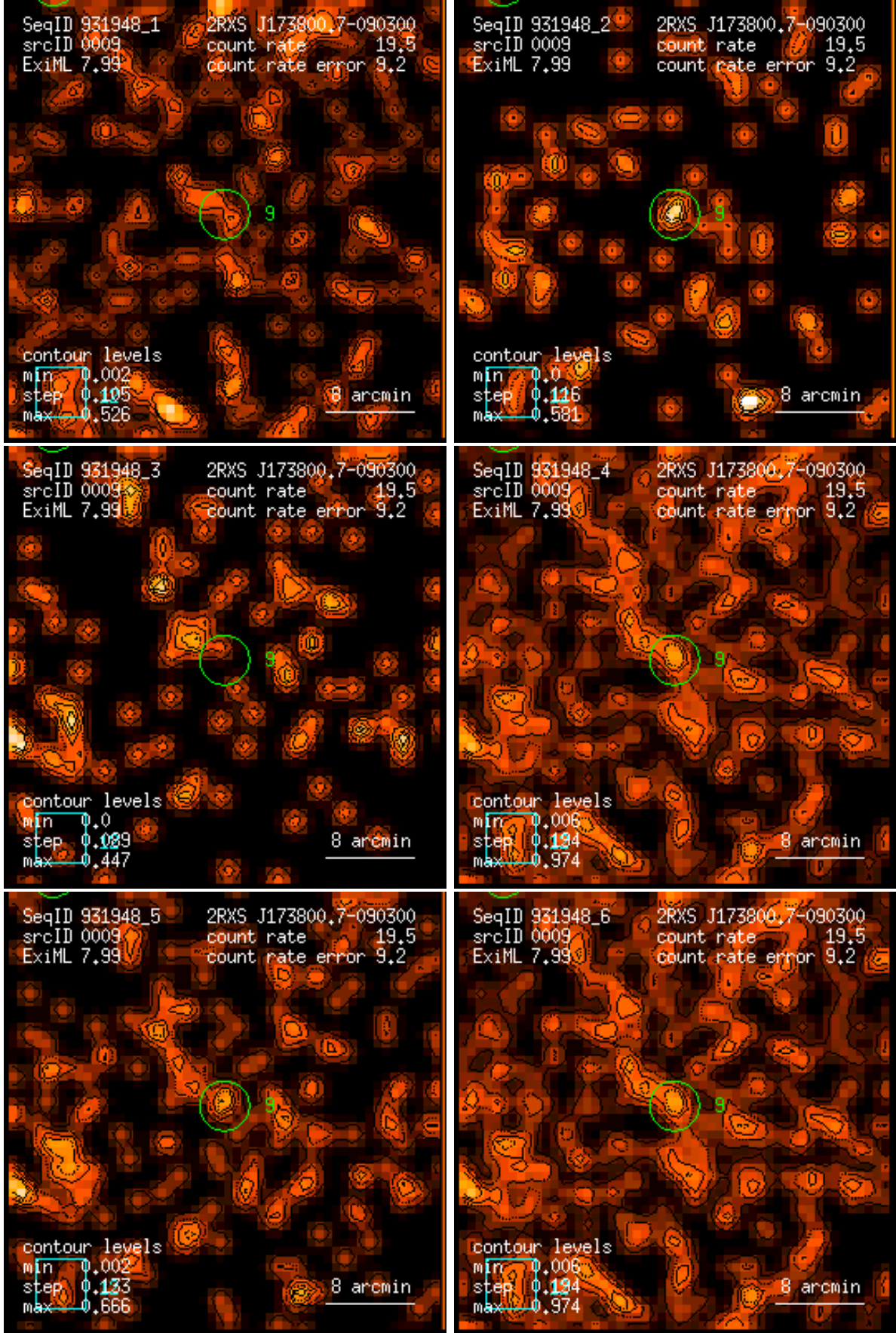
Figure 9: RASS 931948: detection 0009: band rate images, Gaussian filter: (1) PSPC channels 11 – 41, (2) 52 – 90, (3) 91 – 201, (4) 11 – 235, (5) 52 – 201, (6) 11 – 201. Broad band rates in counts/ks. Band rate contour levels in counts/ks/arcmin 2 .
